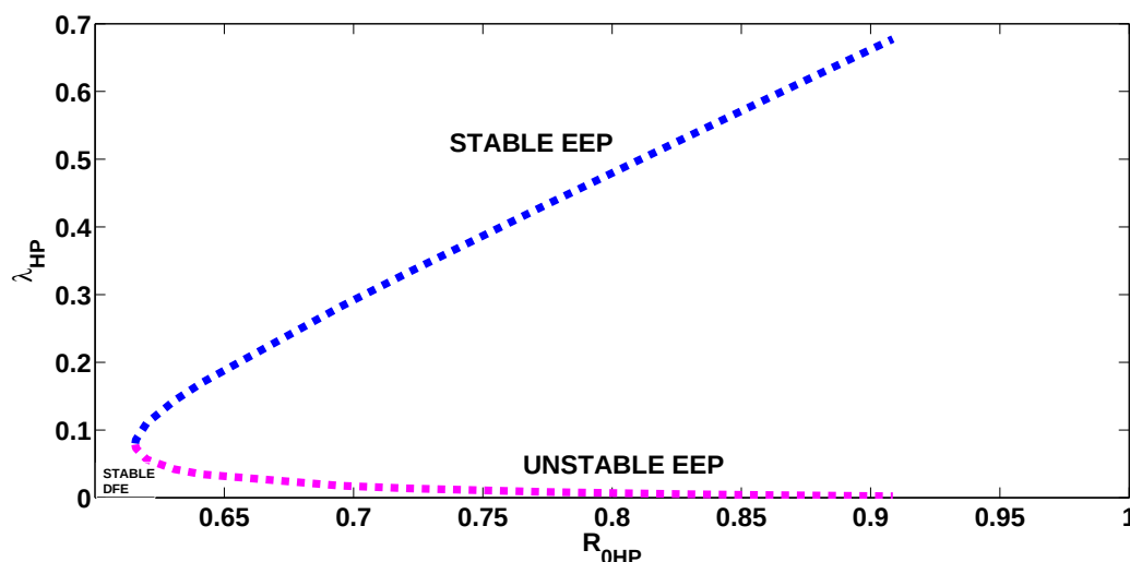
Figure 2: Bifurcation diagram for the HPV-only sub-model (5). Parameter values used are: 1.15168 \leq \beta_{HP} \leq 1.70 , \varepsilon_p = 1.0 . All other parameters as in Table 2
