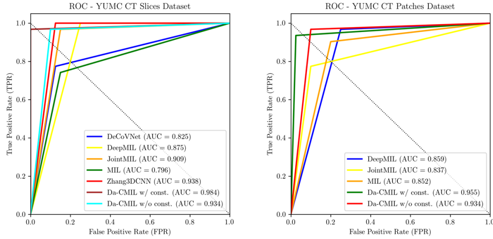
Figure 4: The Receiver operating characteristic(ROC) curves of compared methods on the YUMC CT slices and patch datasets.
