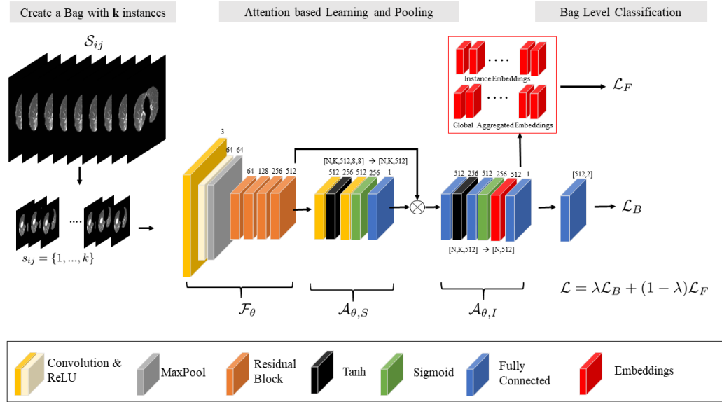
Figure 1: Overview of the proposed framework. For a given patient CT scan, we sample k instances during training to create a bag as input and feed them through the backbone F_\theta to obtain feature maps. Modules A_{\theta,S} and A_{\theta,I} learn spatial and instance attention, then perform permutation invariant pooling via A_{\theta,I} on feature maps to obtain a single bag representation. Prior to pooling, attention-weighted instance features from A_{\theta,I} are employed for unsupervised contrastive learning as well as patient level learning to obtain final predictions and update the model.
