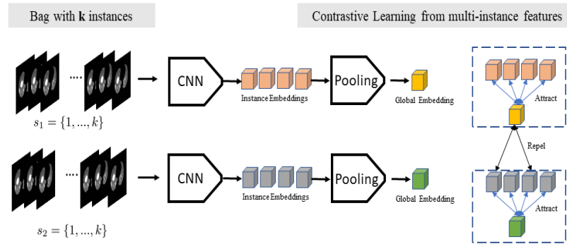
Figure 2: Illustration of contrastive learning applied to the MIL setting during model training.
