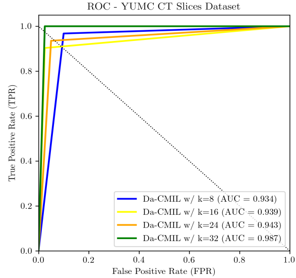
Figure 7: ROC curves of DA-CMIL on YUMC CT Slide dataset when k is varied during training.
