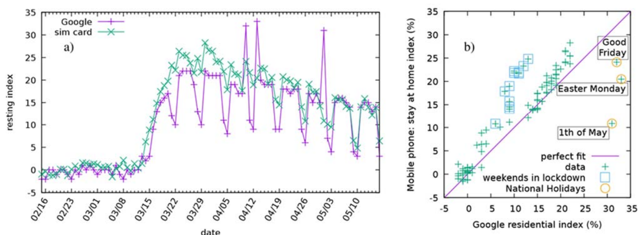
Figure 4. Comparison of two methods for measuring the relative change from the baseline of "staying-at-home". Left (a) : The residential index of Google (purple) and the CDR based stay-at-home index (green) plotted as a time series. Right (b) : Scatter plot of the daily stay-at-home index as a function of the daily residential index of Google. Perfect fit would correspond to a set of points falling onto the diagonal line shown in purple. The weekends during the curfew seem to deviate from this to the left, whereas outliers to the right are corresponding to the national holidays.
