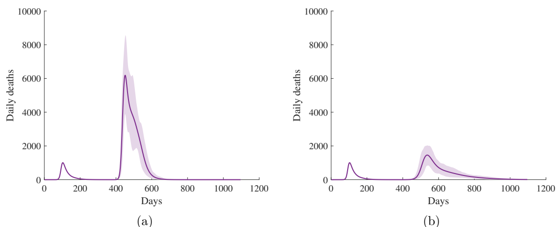
Fig. 3: Projected daily deaths without vaccination given (a) no new control measures leading to R = 2.3(\pm 0.2) , and (b) limited control measures sufficient to reduce the basic reproductive number to approximately R = 1.8(\pm 0.1) . Uncertainty in numbers is represented by the shaded region, within which 95% of simulations are found to fall. Simulations do not include random reintroduction, which may cause a much higher level of uncertainty in the timing of the second outbreak.
