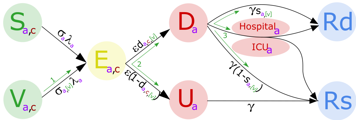
Fig. 1: Representation of model states and transitions. The three different possible types of vaccination are shown by green arrows and bracketed variables. These are:
