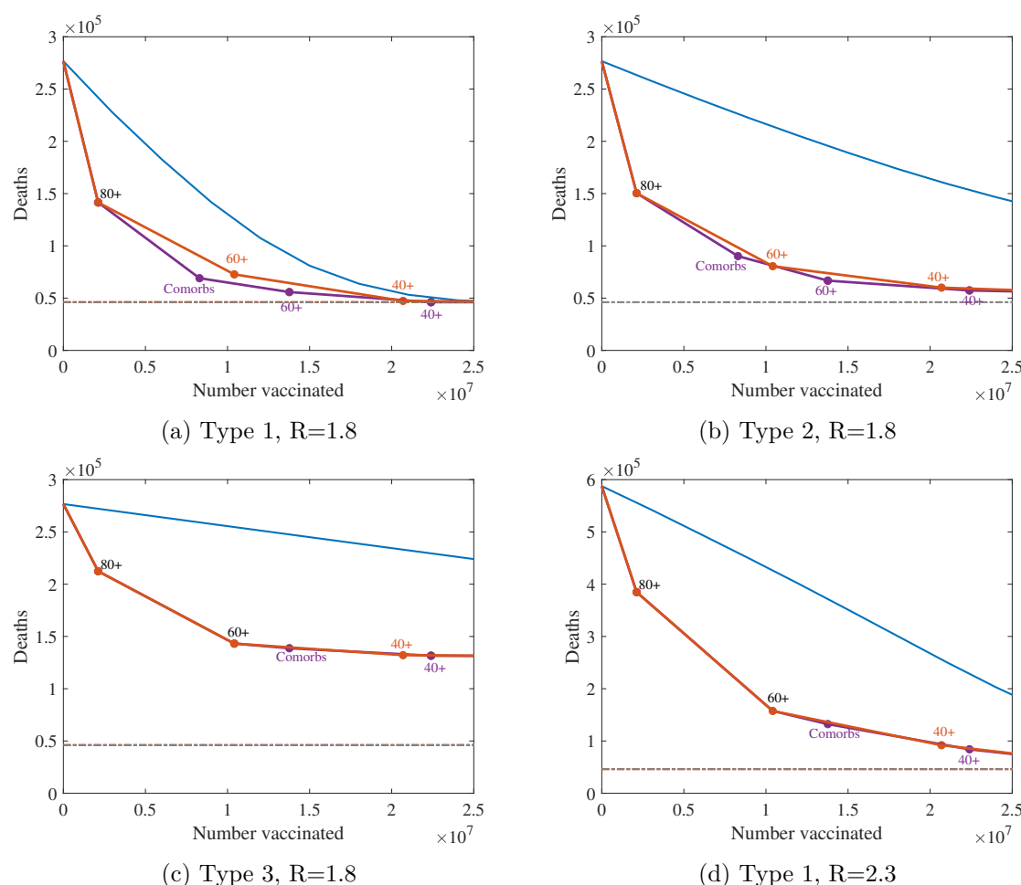
Fig. 4: Comparison of vaccination ordering for four different vaccination scenarios. In each panel, the purple lines show the optimum vaccination ordering of groups comprising of 20 year age bands together with comorbidities across all ages, and the orange line for age groupings only. The optimum strategy is identified by giving greatest reduction in deaths per vaccination in each instance. The blue lines show an unbiased strategy with vaccinated numbers dispersed evenly across the population and the grey dotted line show the base level of morbidity from the first infection wave.
