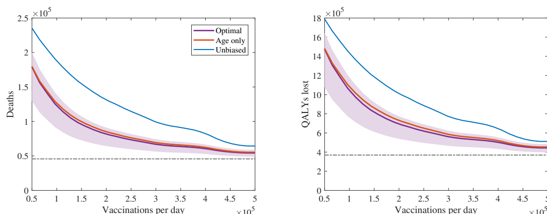
Fig. 7: The total number of (left) deaths and (right) QALYs lost resulting from a second epidemic wave vs speed of deployment for a type 1 vaccination with 70% uptake and 70% efficacy. Vaccine deployment is started 2 months after stricter NPIs are relaxed to leave low level measures sufficient to keep R \approx 1.8 . The purple line (and shaded prediction region) represents projected outcomes under the identified optimal ordering with age and comorbidity groups, the orange line outcomes using the identified optimal ordering accounting for age groups only (without comorbidity), and the blue line outcomes with an unbiased population wide delivery.
