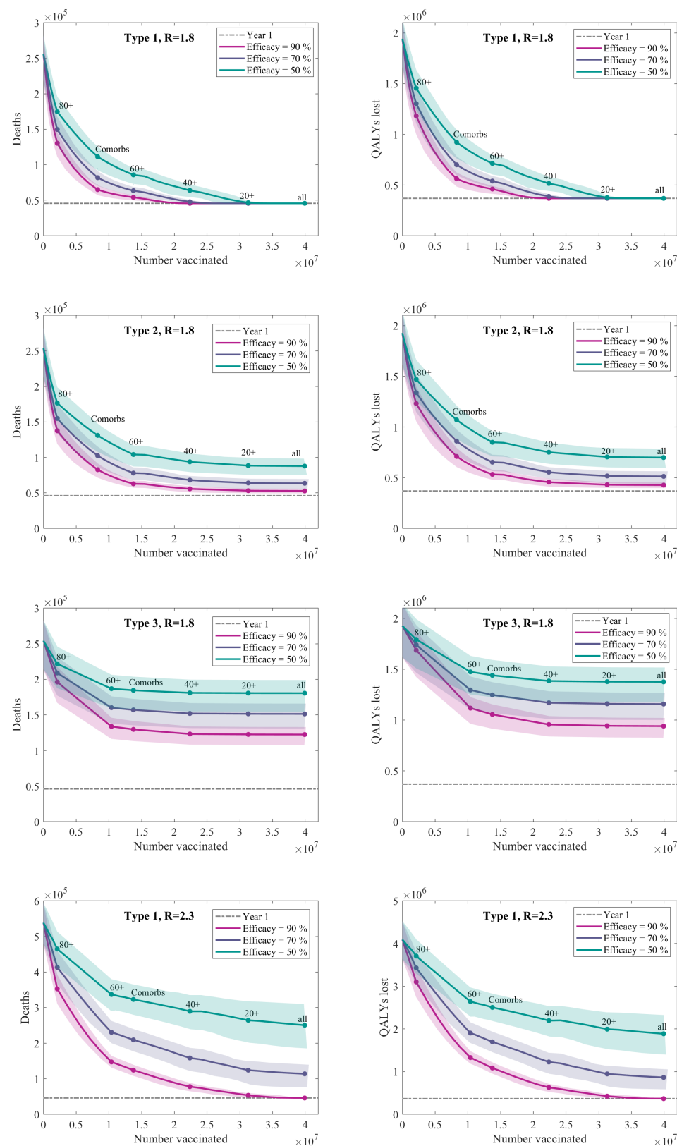
Fig. 6: Deaths and QALYs lost versus the proportion of the population vaccinated. We use the optimal vaccination ordering with a maximum vaccine uptake of 70% across the population. We display the mean values of 100 independent simulations for each vaccine efficacy (solid lines), with 95% prediction intervals (shaded regions). The grey dotted line shows the base level of mortality from the first wave of the pandemic.
