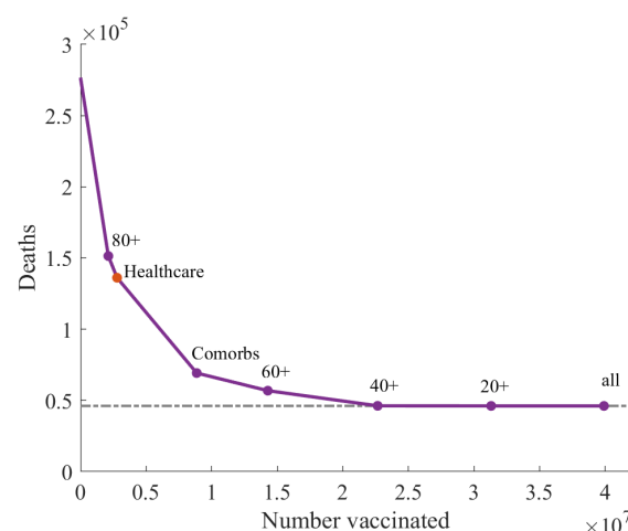
Fig. 5: Optimal vaccination ordering for age, comorbidity and HCW groups in a scenario with a type 1 vaccine and low level social measures ( R = 1.8 ).
