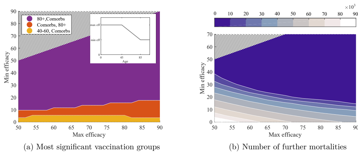
Fig. 8: The effect of different levels of declining type 1 vaccine efficacy ( R \approx 1.8 ) on both the optimal vaccine ordering and success at limiting mortality. A maximum efficacy value is applied to all individuals below the age of 45 and a minimum level to individuals above the age of 85. Efficacy is assumed to decay linearly between these two levels to give the efficacy for intermediary age groups. This distribution is represented by the inset in panel (a). Panel (a) shows when, dependent on minimum and maximum efficacy, the two groups deemed most significant for vaccination impact vary. In the purple region it is optimal to vaccinate those above the age of 80 followed by comorbidities, in the red comorbidities followed by 80+ and in the yellow those in the 40-60 age group followed by comorbidities. Panel (b) shows the expected further mortality resulting from a second infection wave with 70% of the whole population vaccinated for different minimum/maximum type 1 vaccine efficacies. The large dark blue region corresponds to less than 10,000 deaths in any second wave following vaccination.
