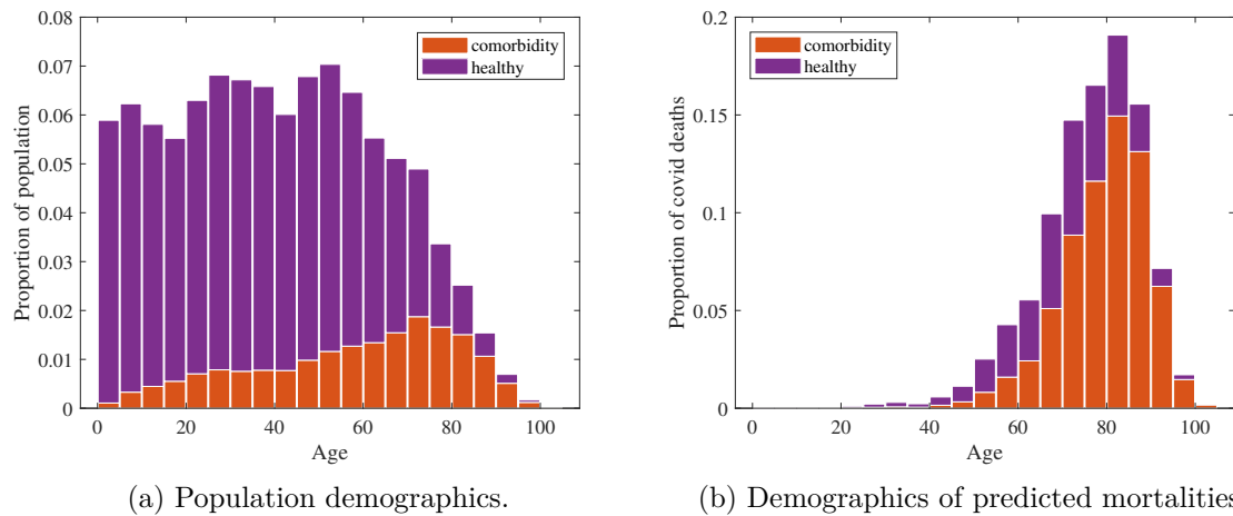
Fig. 2: The percentage of (a) the population and (b) deaths predicted by our model, within each five-year age band. The proportions of each age group with health conditions are shown in red, with the proportion of each age group without health conditions (healthy) shown in purple.
