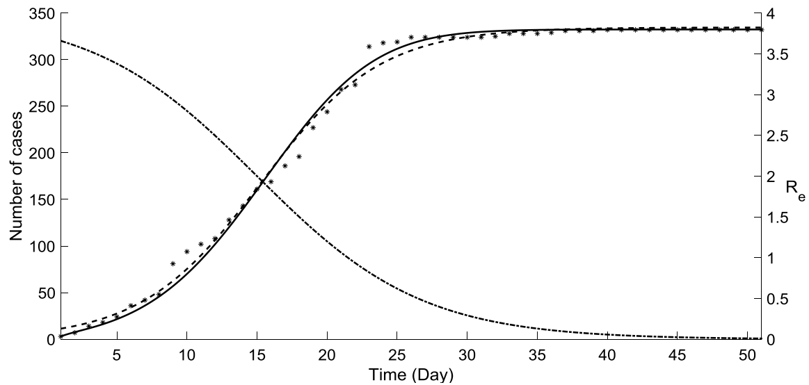
Fig.2. Reported cumulative number of cases in Mauritius (*) and graphical representation of the modelling results: logistic growth (---), SEIQR simulation (full curve) using the optimal effective reproduction number ( -\cdot-\cdot- ) with the parameter values given in the text.
