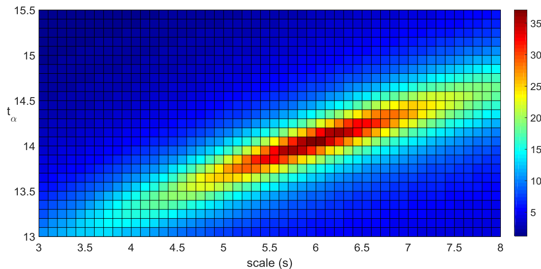
Fig. 3. Comparison of the computed cumulative number of cases using the SEIQR model with the reported number of cases for R_e(0) = 4.0 and varying t_\alpha and s . The colour plot shows the reciprocal of the NRMSE which was used as the comparative statistic.
