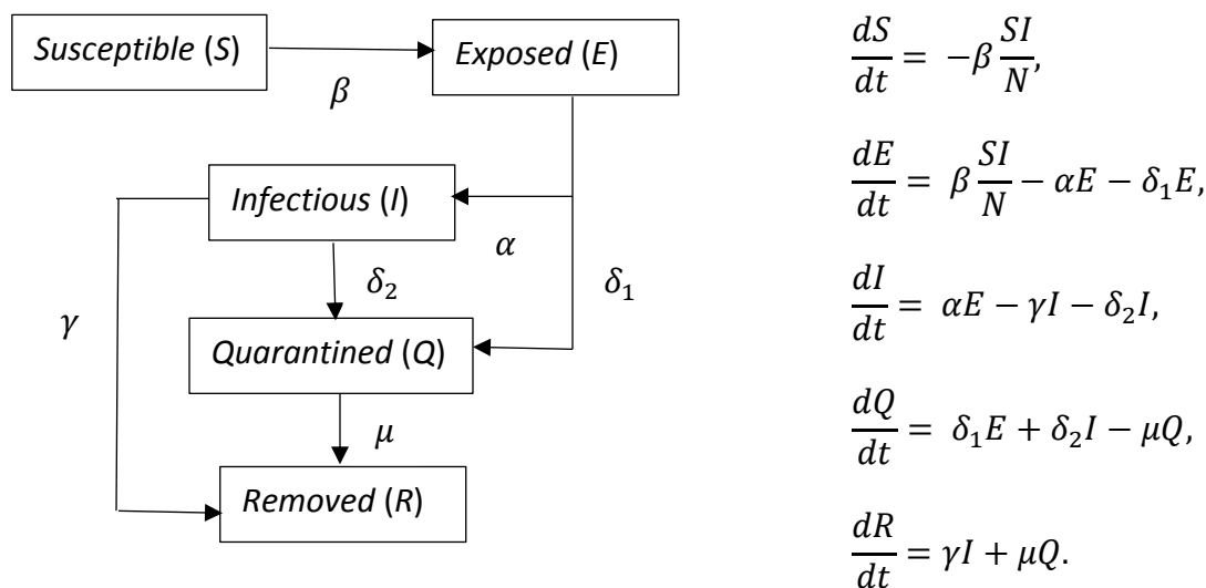
Fig. 1. Schema of the SEIQR model and the dynamical equations used.
