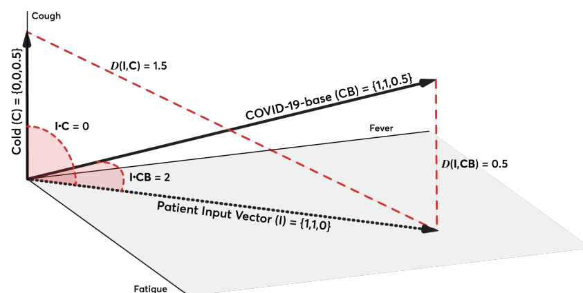
Figure 1. A simplified representation of an input vector from a person with fever and fatigue, but not cough. The Cold and COVID-19-base vectors represent the values of these diagnosis vectors in the dimensions of Fatigue, Fever, and Cough. The red dashed lines represent the Euclidean distances D(X, Y) and the red shaded areas denote the angles \theta that are related to the inner products via \langle X, Y \rangle = \frac{\cos(\theta)}{\|X\| \|Y\|} .
