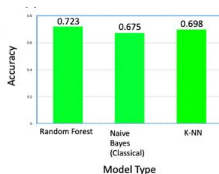
Figure 1. The accuracies of Random Forest, Classical Naïve Bayes, and K-Nearest Neighbor compared. Using a “voting” system, random forest classifiers can quickly learn on data and accurately validate predictions, leading to a higher efficiency and end performance.
