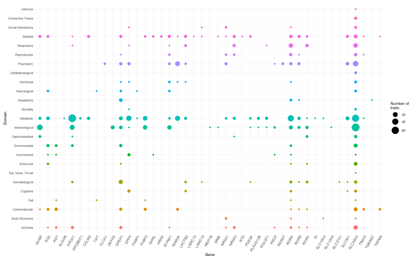
Figure 4: Domain distribution of PheWAS of ACE2-network genes. The ACE2 gene network associations are grouped based on domains (y-axis) and gene names (x-axis). The size of the data points reflects number of phenotypes surviving multiple testing correction.
