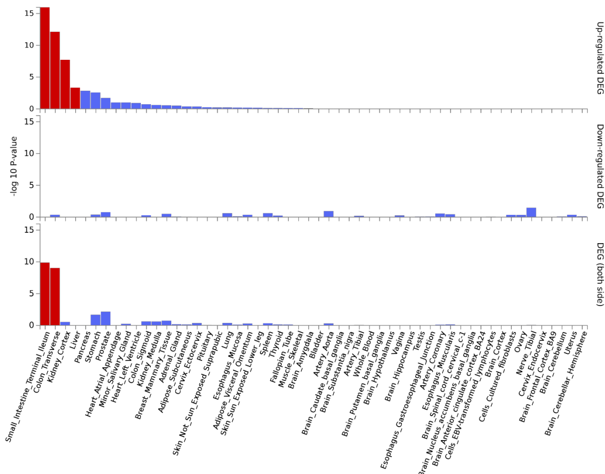
Figure 2: Tissues enriched based on ACE2-network gene expression for GTEx tissues. The genes from the ACE2-network show over-representation of tissues (x-axis) and -\log_{10} p\text{-value} (y-axis). The red bars are significant enrichments.
