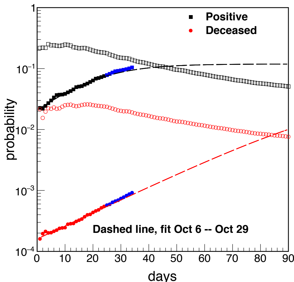
Figure 2. Same as figure 1 but for the probabilities given by the number of cases divided the number of tests [1]. Fits are obtained using eq.(1), no decay stage is observed yet, opposite to the Spring data (open symbols).
