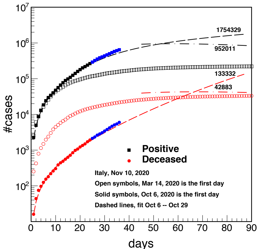
Figure 1. Number of cases vs. time in days in Italy. The open symbols refer to the effective data registered starting from March 14 th , 2020: the lockdown day. The full symbols refer to data starting from October 6 th . The dashed lines are from the fits, eqs.(1-3).
