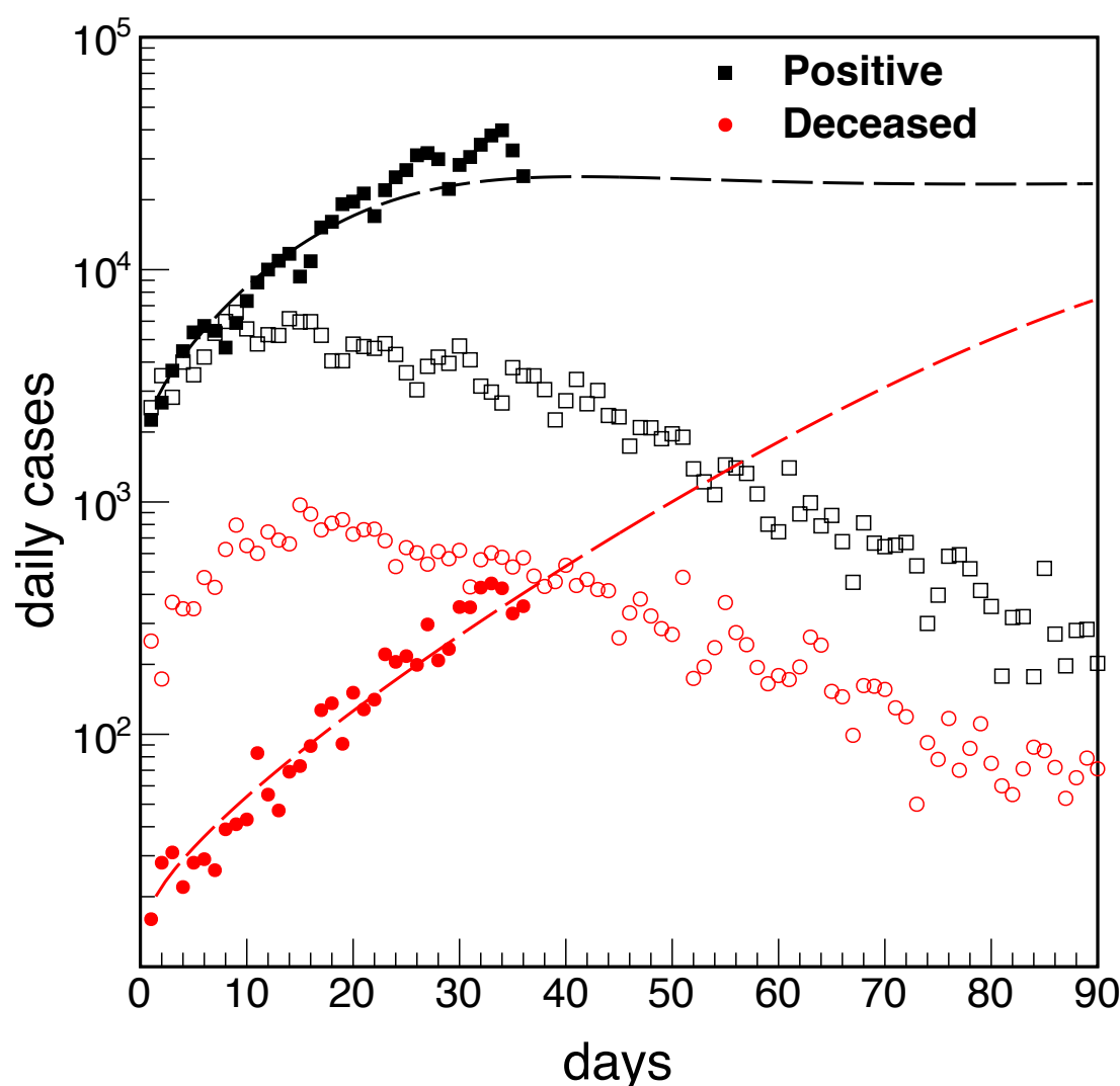
Figure 3. Number of daily cases vs time, symbols as in figure 1. This quantity can be obtained from the time derivative of the quantities reported in figure 1 or from data directly (open and full symbols).
