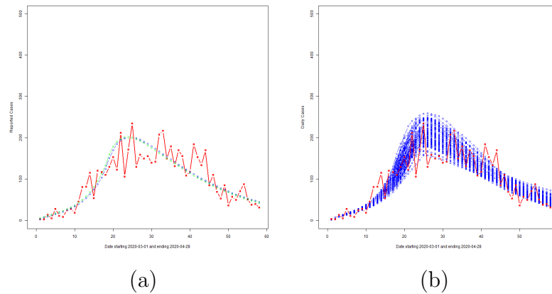
Figure 9: Effect of redistribution: Panel (a) shows the redistributed daily cases and the corresponding best fit curves of \gamma_o I_o(t) (blue line) and \Delta R_o(t) (green line) based on \hat{\Theta}_{MAP} . Panel (b) shows the variability of the fit based on the ensemble set \{\Theta_i^*\}_{i=1}^M .
