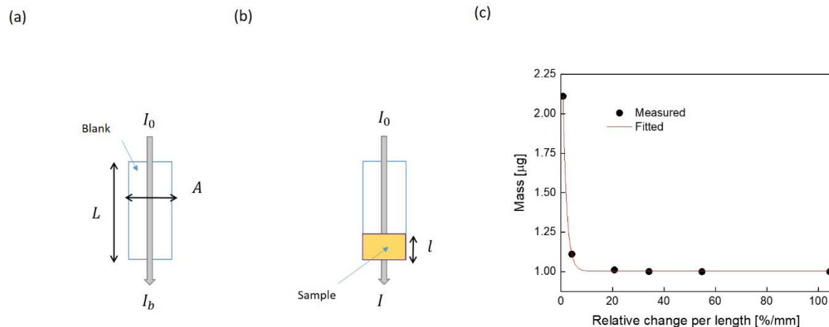
Figure 4: Illustration of light intensity and its path length: (a) the blank representation, and (b) light path length of the sample. L and A are the length and cross-sectional area of container, l is the light path length. I_0 , I_b and I are the incident, blank and instantaneous sample intensities, respectively. (c) Loaded mass versus relative change in light intensity per light-path length. The measured points were fitted with exponential function expressed by
