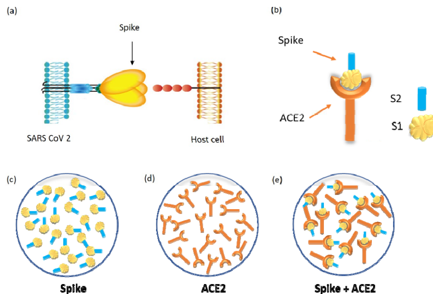
Figure 1: Schematic illustration of SARS-CoV-2 spike protein and ACE2 receptor binding. (a) SARS-CoV-2 binding to the ACE2 receptor on the host cell surface. (b) Binding of ACE2 and spike protein along with illustration of the spike protein subunits, S1 and S2. (c) Schematic showing the distribution of the spike protein in solution. (d) Schematic showing the distribution of ACE2 in suspension. (e) Distribution of ACE2 and S protein after binding in solution.
