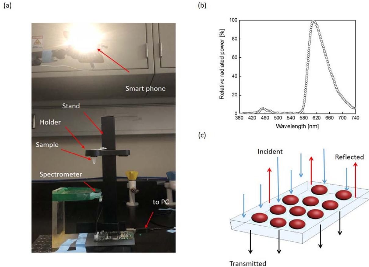
Figure 2: The proposed concept of optical detection and the experimental design: (a) The optical measurement setup is shown consisting of a smart phone as a light source and the mini-spectrometer utilized to collect the light waves passing through the sample kept in the holder. (b) The smart phone power spectra versus wavelength. (c) Illustration of the spectrometer detection principle.
