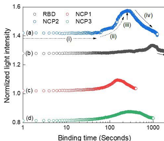
Figure 9: Optical profiles for normalized interactions versus binding time under different conditions for RBD and NCP. (a) NCP with its antibody at the maximum concentration of 22 \mu\text{g} per ml (b) RBD with its antibody, (c) NCP with its antibody at a 1:10 dilution (d) NCP with its antibody at 1:10 with outside mixing.
