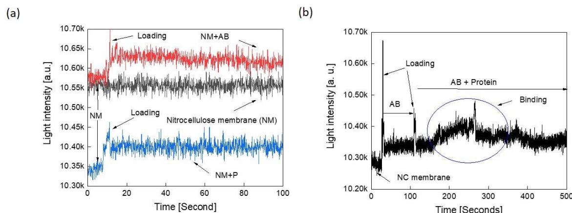
Figure 7: Test of protein-protein interaction measurements on solid support: (a) Optical responses on nitrocellulose membrane (NM) alone, nitrocellulose membrane and spike protein (NM+P), and nitrocellulose membrane and antibody to spike protein (NM+AB) alone. (b) Optical responses to spike protein-antibody binding on the nitrocellulose membrane.
