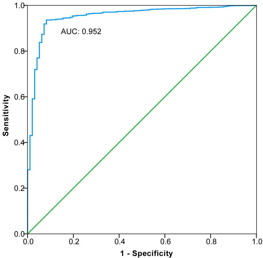
ROC Curve
