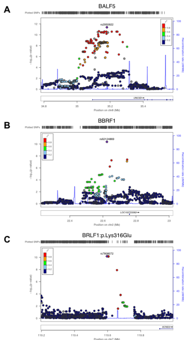
Figure 3: Locuszoom plots.
