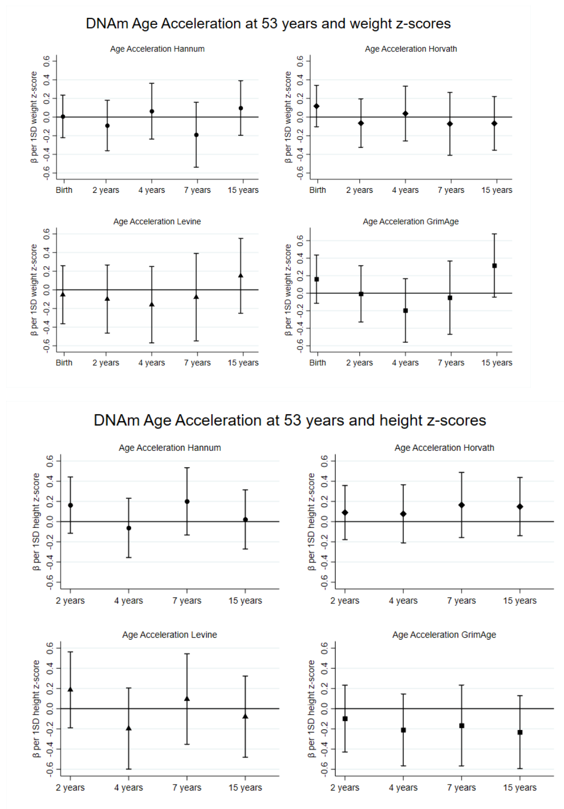
Figure 1. Preliminary results for DNAm Age Acceleration at 53 years and weight and height z-scores. Adjusted for height/weight z-score, age in months at 53 years and sex. Each coefficient represents mean change in AgeAccel (y) for a 1 SD increase in height/weight. Separate analyses were conducted at each age.
