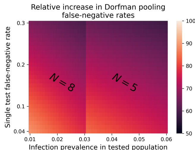
Figure 1: Relative increase in Dorfman pooling false-negative rates E_{\text{rel}} . Color represents the relative percentage increase in the scheme false-negative rates relative to the single test false-negative rates, P_{\text{fn}} . The disease prevalence, q , is varied on the x-axis, while the single test false-negative rate is varied on the y-axis. Note that Pool size, N , was chosen according to q as in [1].
