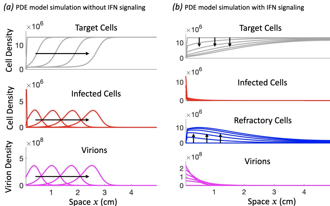
Figure 2: Model simulations show that paracrine IFN signaling strongly interferes with the spatial spread of infection. Shown is the solution of the model system at successive time points, with arrows indicating the direction of progression with time. (a) A representative simulation of the PDE model with k = \pi = 0 (no IFN), exhibiting traveling wave behavior initiated from a single nexus of infected cells at position x = 0 . The infection travels an equal distance between successive times, demonstrating constant speed of spread. (b) A representative simulation of the PDE model with cell protection included ( \pi \neq 0 ) showing how IFN signaling can stop the spread of infection by depleting target cells. The distribution of virions and infected cells can be seen to remain localized to the left side of the domain, as the rapid depletion of susceptible cells (as a result of increases in refractory cell population) in the domain prevent the infection from establishing a traveling wave.
