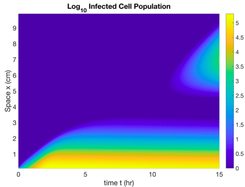
Figure S2: Given sufficient time, infection will reemerge despite strong IFN signaling. Shown is a representation of \log_{10} I(x, t) over sufficient time scale for infection to reemerge far from initial location. This phenomenon is an artifact of the continuum approximation inherent in the PDE fomulation of the model. Due to the parabolic nature of the PDE, compact data becomes immediately non-zero in the entire domain, leading to inevitable reemergence of infection in locations where only fractional amount of virus is present.
