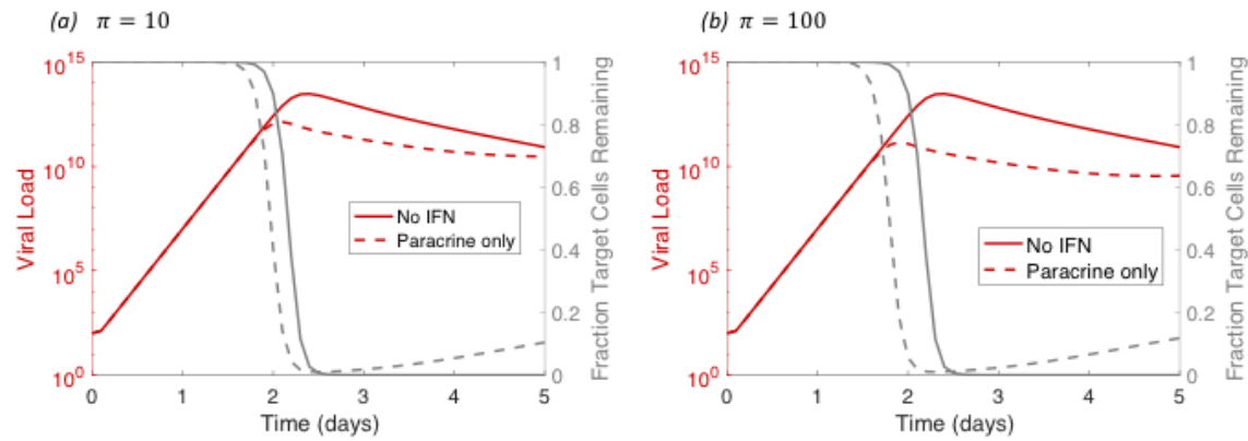
Figure S1: Even supraphysiological levels of IFN production \pi do not affect initial exponential growth rate. Very high levels of free IFN can shorten the time to peak viremia, but do not demonstrate the ability to halt establishment of systemic infection.
