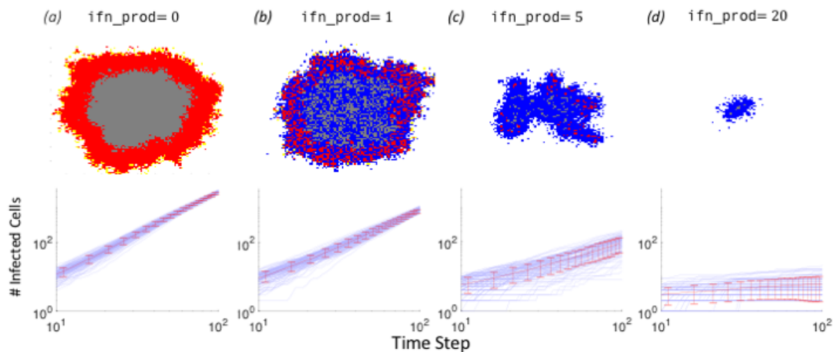
Figure 4: High production of IFN ( ifn_prod ) interferes with or stops the spread of infection by insulating infected cells from target cells with a layer of refractory cells. Top row shows example of simulations of the cellular automata (CA) model at 100 time steps on a 100 \times 100 grid. Bottom row shows log-log plots of the number infected cells verses time for 100 independent simulations of CA with mean and standard deviation plotted in red. The approximate linear trend shown on the log-log plots suggests that the number of infected cells fits roughly a power law in time, I(t) \propto t^\gamma , where \gamma is the slope of the trend line. For ifn_prod = 0 and 1, \gamma is approximately 2, consistent with a traveling wave solution of the PDE model. \gamma decreases as ifn_prod increases. In the images of the CA grid, red, blue and gray dots indicate infected cells, refractory/protected cells and dead cells, respectively; Target cells are left white.
