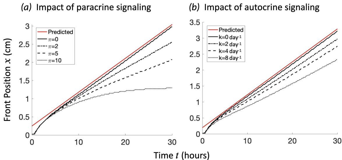
Figure 3: Comparison of the impacts of paracrine signaling and autocrine signaling on viral spatial spread. Shown is the position x(t) of the infection front over time for various values of the IFN production parameter \pi while keeping k = 0 and the autocrine-mediated transition rate k while keeping \pi = 0 . Here we define the front position x(t) to be the position that 1% of total cells are infected, i.e. I(x(t), t) = 0.01T_0 . (a) Sufficiently strong paracrine signaling, e.g. setting \pi = 10 and k = 0/\text{day} , leads to halting the spread of infectious front. (b) Strong autocrine signaling, e.g. setting \pi = 0 and k = 8/\text{day} , impact modestly on the speed of the viral spread. The red lines show the predicted front position given the analytically derived wave speed in Eqn. (3).
