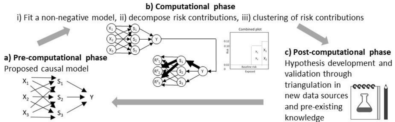
Figure 1. The phases of the CoOL approach towards inference to the best explanation
