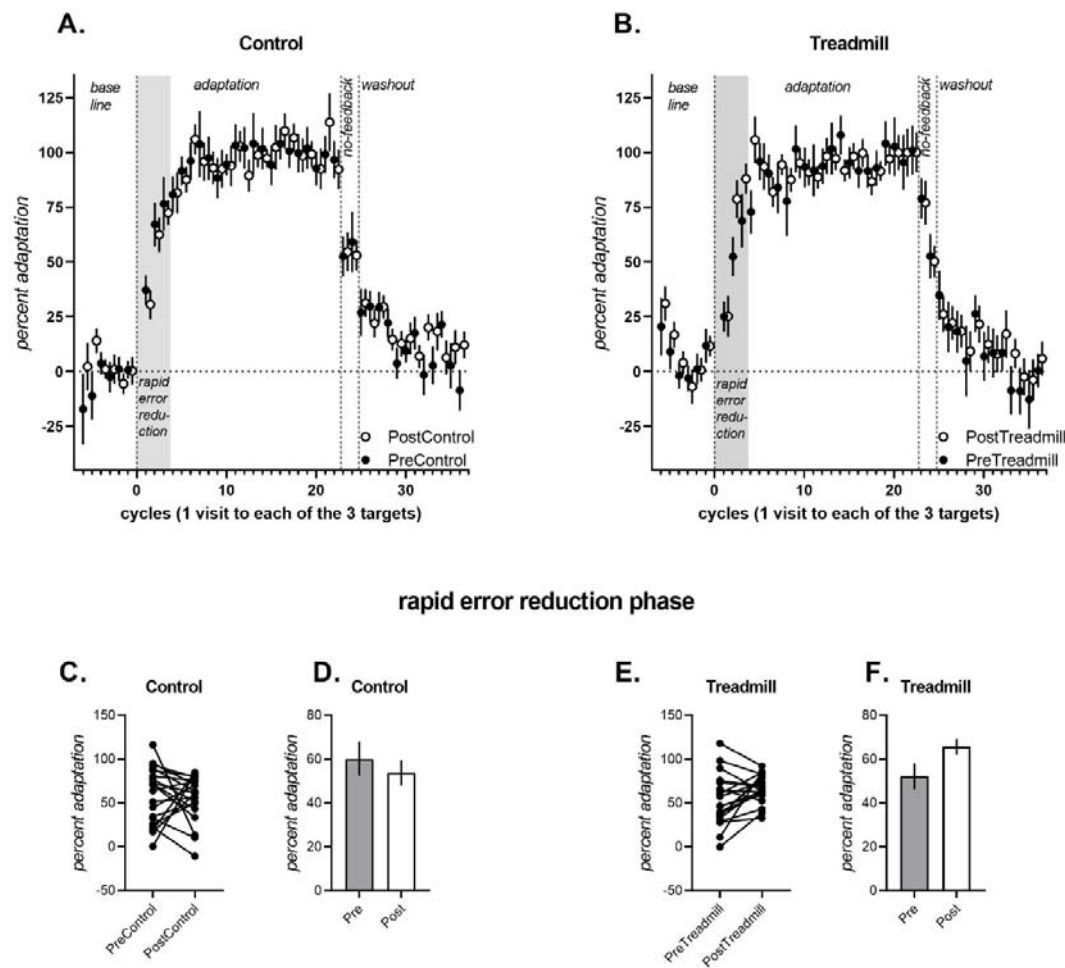
Figure 2: Percent adaptation of participants during the adaptation (cycles 1-22), no-feedback (cycles 23-24) and washout (cycles 25-36) trials for the control condition (A) and the exercise condition (B). Note that data from the Post conditions are offset by 0.5 to avoid being obscured by data from the Pre conditions. There was a significant interaction between the control and exercise condition from pre to post in the rapid error reduction phase (shaded region, i.e., first 3 adaptation cycles). Individual participant data in the rapid error reduction phase is shown for the control condition (C) and the treadmill condition (E). Covariate adjusted mean percent adaptation for the rapid error reduction phase is shown for the control (D) and treadmill (F) conditions
