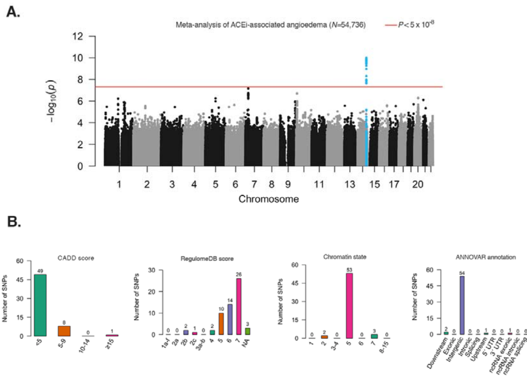
Figure 1. SNP-based results from the genome-wide association study (GWAS) meta-analysis on ACE-inhibitor associated angioedema in 54,736 individuals. A. Manhattan plot of the GWAS meta-analysis of ACE-inhibitor associated angioedema, showing the negative log 10 -transformed P -value for each SNP. P -values were obtained from a logistic regression mixed model. B. Distribution of CADD scores, RegulomeDB categories, chromatin state and functional consequences of all annotated SNPs in linkage disequilibrium ( r^2 \geq 0.6 ) with the lead GWAS SNPs.
