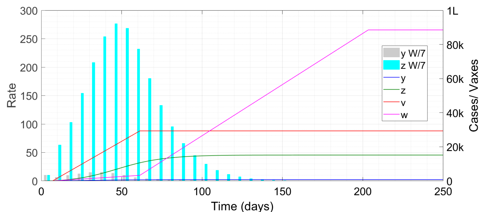
Figure 3 : Time trace of the epidemic with vaccination. The symbol 'k' denotes thousand, 'L' hundred thousand and 'W/7' weekly cases scaled down by a factor of seven.
