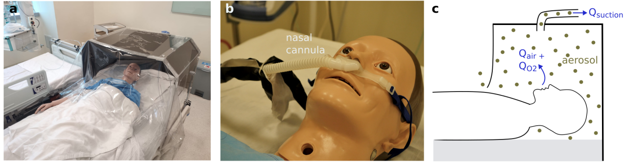
FIG. 1. (a) Barrier enclosure used to contain aerosols from patients who typically require supplementary oxygen treatment (b) delivered through a nasal cannula. (c) For effective containment of aerosol (gray dots), the suction rate Q_{\text{suction}} must be higher than the oxygen flow rate Q_{\text{O}_2} and the breathing (expiration) rate of the patient Q_{\text{air}} combined.
