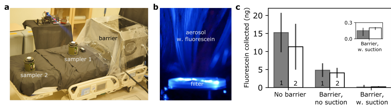
FIG. 3. (a) To quantify the amount of aerosol leak, we placed two air samplers outside the barrier enclosure. (b) Aerosol droplets (with added fluorescein) were trapped by the filter on the air sampler, which can then be detected using spectrofluorometer. (c) The amount of fluorescein collected by air samplers 1 and 2 for enclosure barrier with and without suction can then be compared to the control, i.e. no barrier. Error bars are the standard deviation for triplicates.
