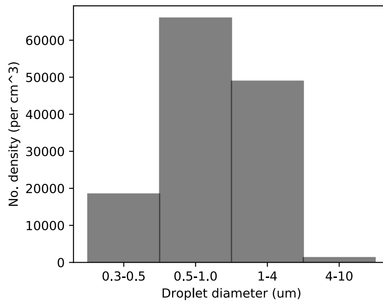
FIG. S2. Droplet size distribution measured using an optical particle sizer.
