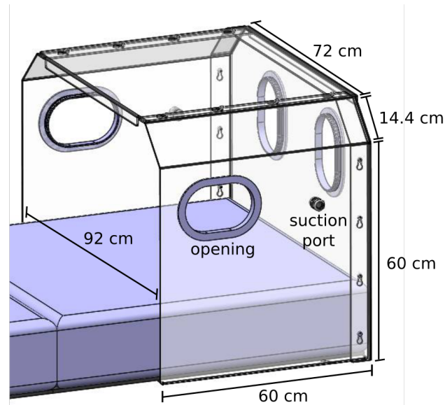
FIG. S1. Barrier enclosure design
