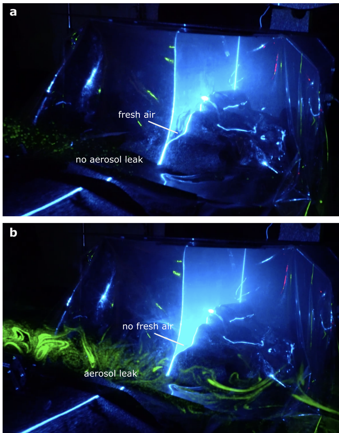
FIG. S3. Visualization of aerosol flow (a) with and (b) without suction.
