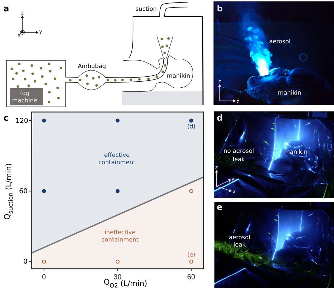
FIG. 2. (a) Experimental setup used to simulate the breathing cycle. Nasal cannula used to deliver oxygen not shown. (b) Micron-sized glycerin-water aerosol droplets expelled from the manikin can be visualized by shining a blue laser sheet at the sagittal plane. (c) Effectiveness of aerosol containment depends on the applied suction rate Q_{\text{suction}} and the oxygen flow rate Q_{\text{O}_2} . Blue filled dots and red unfilled dots correspond to experimental conditions resulting in effective and ineffective containment, respectively. (d) An additional green laser sheet (transverse x - z plane) placed outside the enclosure is not visible in the absence of aerosol leak. (e) Aerosol leaking out from the enclosure scatters light and renders the green laser sheet visible. Experimental conditions corresponding to (d) and (e) are indicated in the phase diagram in (c).
