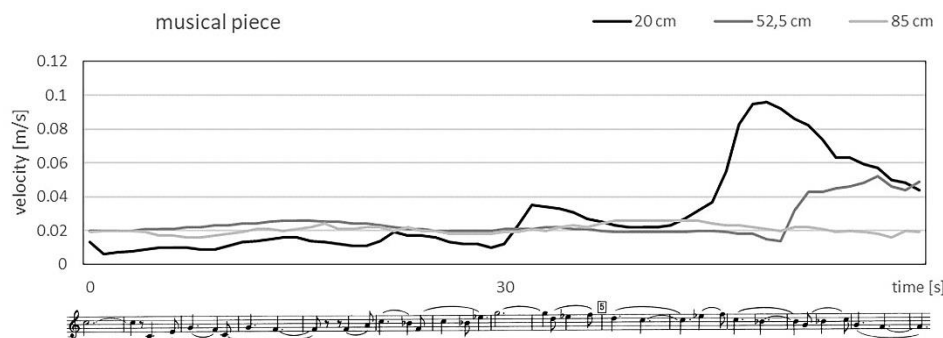
Fig. 6 Velocity of the air escaping from the bell of the oboe when playing Bohuslav Martinů: Concerto for Oboe and Small Orchestra
