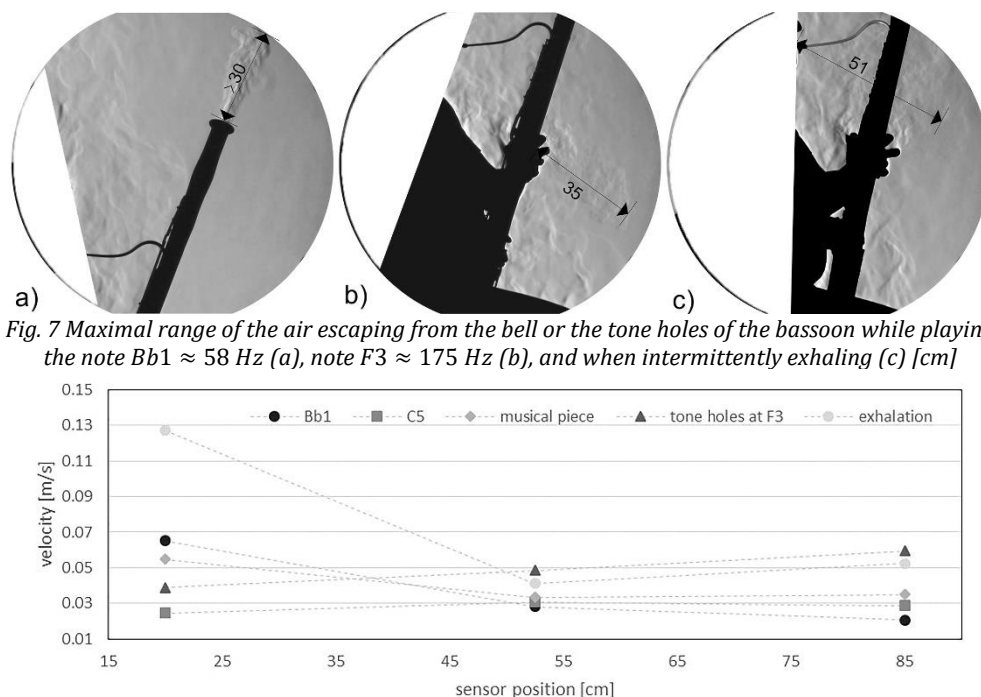
Fig. 7 Maximal range of the air escaping from the bell or the tone holes of the bassoon while playing the note Bb1 \approx 58 Hz (a), note F3 \approx 175 Hz (b), and when intermittently exhaling (c) [cm]
