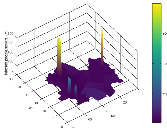
Figure 18: Infected people after 200 time-steps q = 0
