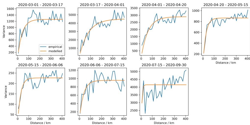
Figure 9: The empirical and the modelled exponential variograms of the cumulative rates of reported cases for every NPI period. The variance is proportional to the cases and the flattening of the exponential variograms indicates the correlation length.
