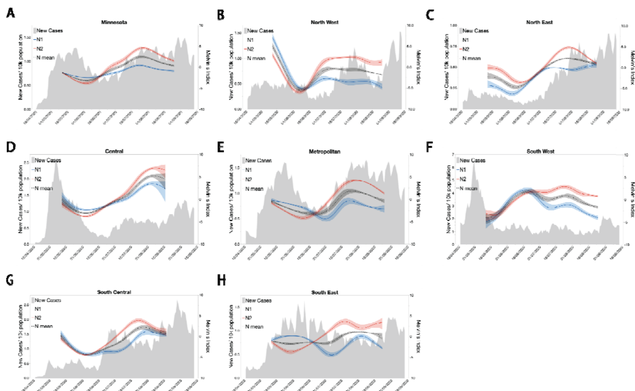
Figure 4. Trends for indexed wastewater SARS-CoV-2 levels across the state show a similar pattern to that of new cases per capita with a temporal offset. A) New clinical cases of COVID-19 overlayed by the indexed SARS-CoV-2 N1, N2, and the mean of N1 and N2 data from RT-qPCR analysis of wastewater samples collected across the state of Minnesota from May to September. B, C, D, E, F, G, H) New clinical COVID-19 cases overlayed by indexed SARS-CoV-2 N1, N2, and the mean of N1 and N2 data from RT-qPCR analysis of wastewater collected from different regions of the state of Minnesota.
