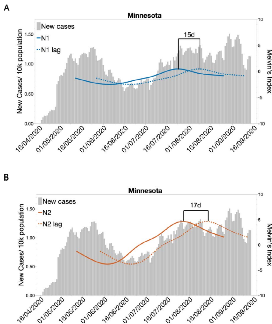
Figure 5. Indexed SARS-CoV-2 levels in municipal wastewater predict new clinical cases in Minnesota. A) Correlation and lag analysis of wastewater SARS-CoV-2 N1 levels with new clinical cases of COVID-19 for the state of Minnesota. B) Correlation and lag analysis of wastewater SARS-CoV-2 N2 levels with new clinical cases of COVID-19 for the state of Minnesota. ***, indicates p < 0.001
