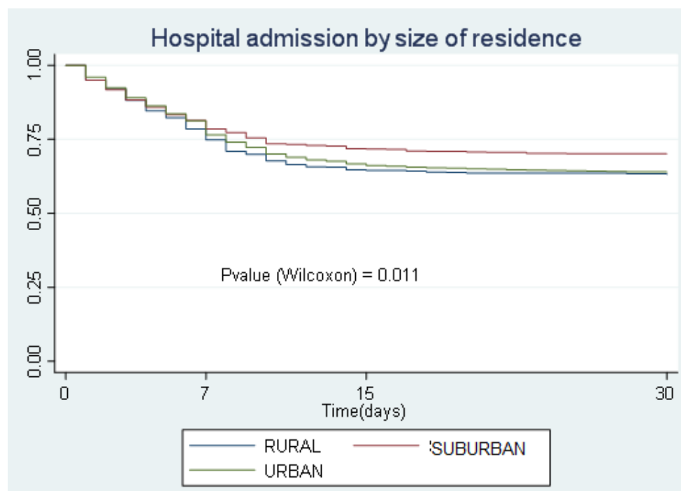
Figure 1: Hospital admission by size of residence, Kaplan–Meier survival
