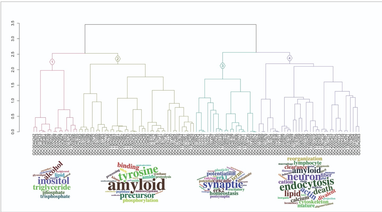
Figure S4: Hierarchical clustering of the semantic similarity matrix and the 4 functional clusters' definition.
