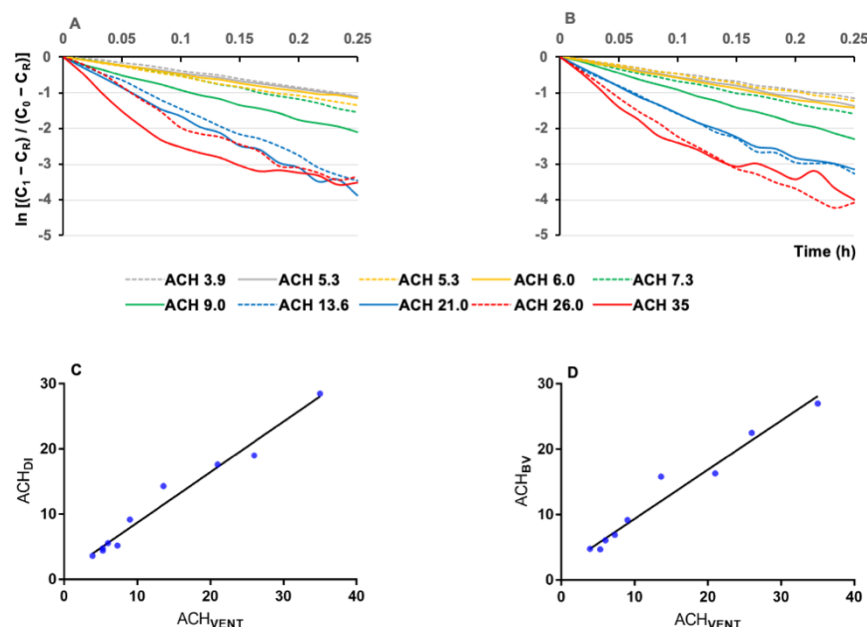
Figure 3. A: CO 2 decay constants by dry ice, B: CO 2 decay constants by baking soda and vinegar; C and D: association between mechanical ventilation rates measure by air flow (ACH VENT ) and ventilation rates measured by CO 2 decay using dry ice (ACH DI ) and baking soda and vinegar (ACH BV ) in dental treatment rooms. Rooms with high mechanical ventilation rates showed rapid decrease of CO 2 concentrations over time (A, B). Both ACH DI and ACH BV are linearly correlated with ACH VENT (C, D).
