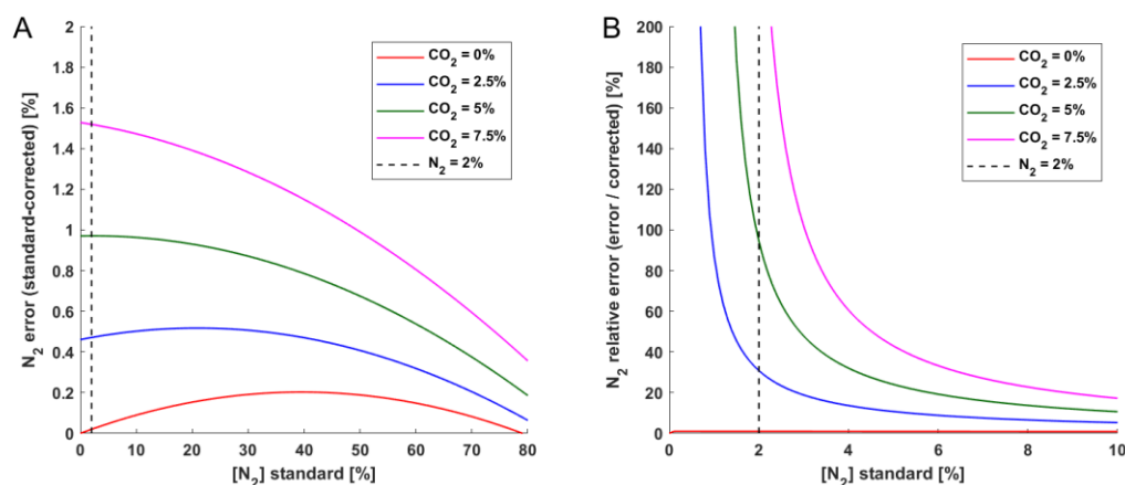
Figure 3: N 2 error as a function of measured N 2 . Illustration of the impact of the O 2 and CO 2 correction functions on final measured N 2 . A) Summed up correction functions of Figure 1 and Figure 2, and therefore absolute error in N 2 , represented as curve for selected concentrations of CO 2 . B) Relative error in measurement of N 2 (standard-corrected/corrected) as a function of N 2 .
