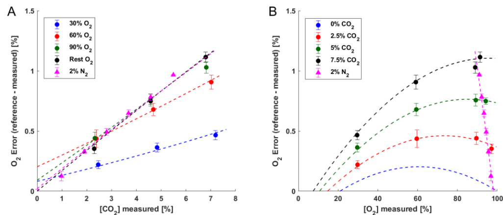
Figure 1: Observed absolute error between known reference and measured O 2 concentrations. (dots: mean of error for one gas mixture, error bars: +/- SD of error). Curves represent a two parameter quadratic polynomial fitted through the error values (see OLS for details), represented here as curves for given CO 2 or O 2 concentrations. Dots represent measurements performed with 12 technical gas mixtures as reference, triangles represent mass spectrometry reference measurements of 6 mixtures at the end of test condition (2% N 2 ). A) Absolute O 2 error as a function of CO 2 concentration, B) Absolute O 2 error as a function of O 2 concentration. Dashed curves all represent the same fit f(O_2, CO_2) .
