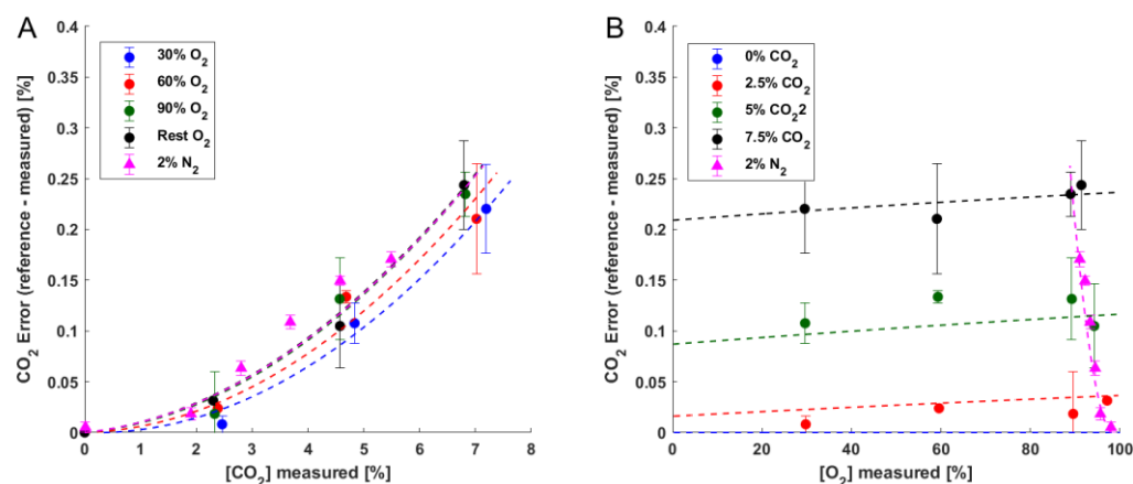
Figure 2: Observed absolute error between known and measured CO 2 concentrations. (dots: mean of error of one gas mixture, error bars: +/- SD of error). Curves represent a two parameter quadratic polynomial fitted through the error values (see OLS for details), represented here as curves for given CO 2 or O 2 concentrations. Dots represent measurements performed with 12 technical gas mixtures as reference, triangles represent mass spectrometry reference measurements on 6 mixtures at the end of test condition (2% N 2 ). A) Absolute CO 2 error as a function of CO 2 concentration, B) Absolute CO 2 error as a function of O 2 concentration. Dashed curves all represent the same fit f(O_2, CO_2) .
