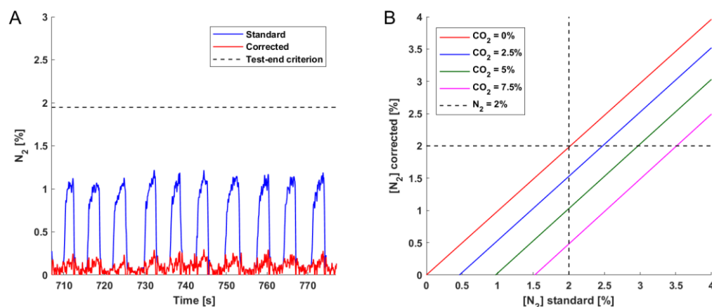
Figure 7: Illustration of the effect of the sensor correction function on nitrogen measurement in the late phase of MBW tests. A) Example of the equilibrium N_2 reached in a very long continued MBW measurement using the Exhalyzer D, displaying a greatly decreased N_2 -back-diffusion equilibrium (tissue nitrogen). B) Corrected N_2 plotted against standard N_2 in conditions around the end of test condition (2% N_2 ).
