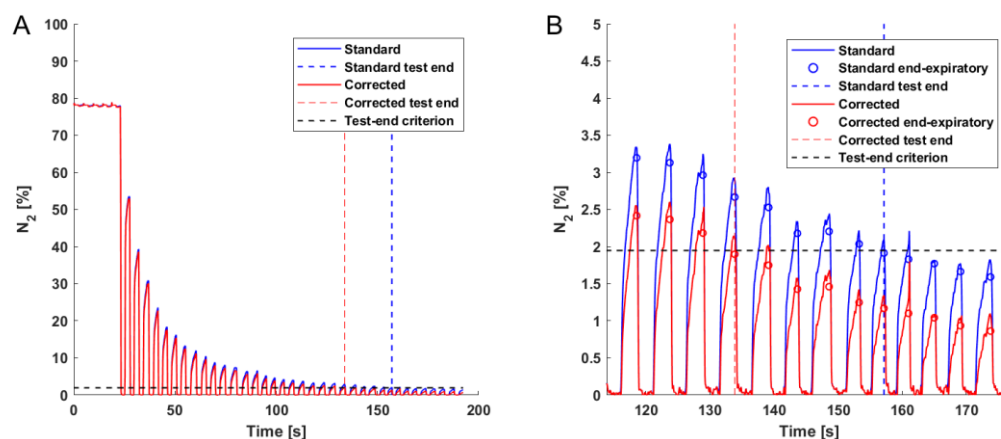
Figure 4: Illustration of the effect of the sensor correction on the N_2 signal and consequently on the end of test of an example MBW measurement. Traced in blue is the signal output of the standard signal processing, corrected signal is shown in red. Vertical dashed lines represent the end of test for the current standard and corrected measurement respectively. The black line corresponds to 1/40^{\text{th}} of the initial N_2 concentration (end of test criterium). A) Time course of N_2 throughout a standard MBW measurement. B) Zoom into the critical period of end of test determination. In this example the test ends 5 breaths earlier in the corrected measurement compared to standard.
