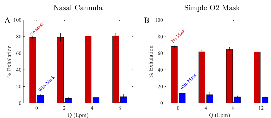
Figure 5: The percent of breath that is exhaled above the face without and with surgical mask as a function of flow rates for (A) the nasal cannula and (B) the simple O2 mask. All cases have five trials.
