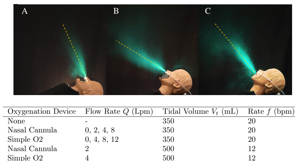
Figure 1: The time averaged exhalations emerging from the nose of a medical manikin fitted with a nasal cannula when the head rests flat (A), and while it is on a bed propped at 45 degrees (B), and when exhaling through the mouth (C), under shortness of breath conditions ( V_t = 350 mL at f = 20 bpm; Q = 4 Lpm). The aerosol-laden exhalation is visualized with back lighting and rendered with artificial cyan coloring. A primary turbulent exhalation jet is observed which spreads conically with principal direction indicated with dashed line with elevation angle \theta = 60 \pm 0.5 degrees (A), 19.3 \pm 0.5 degrees (B), and 56 \pm 1 degrees (C). Table: Summary of the oxygenation devices, flow rates, and breathing tidal cycles investigated ( Q = 0 Lpm cases were conducted for calibration purposes). Corresponding movies found in SI Movie 1-3.
