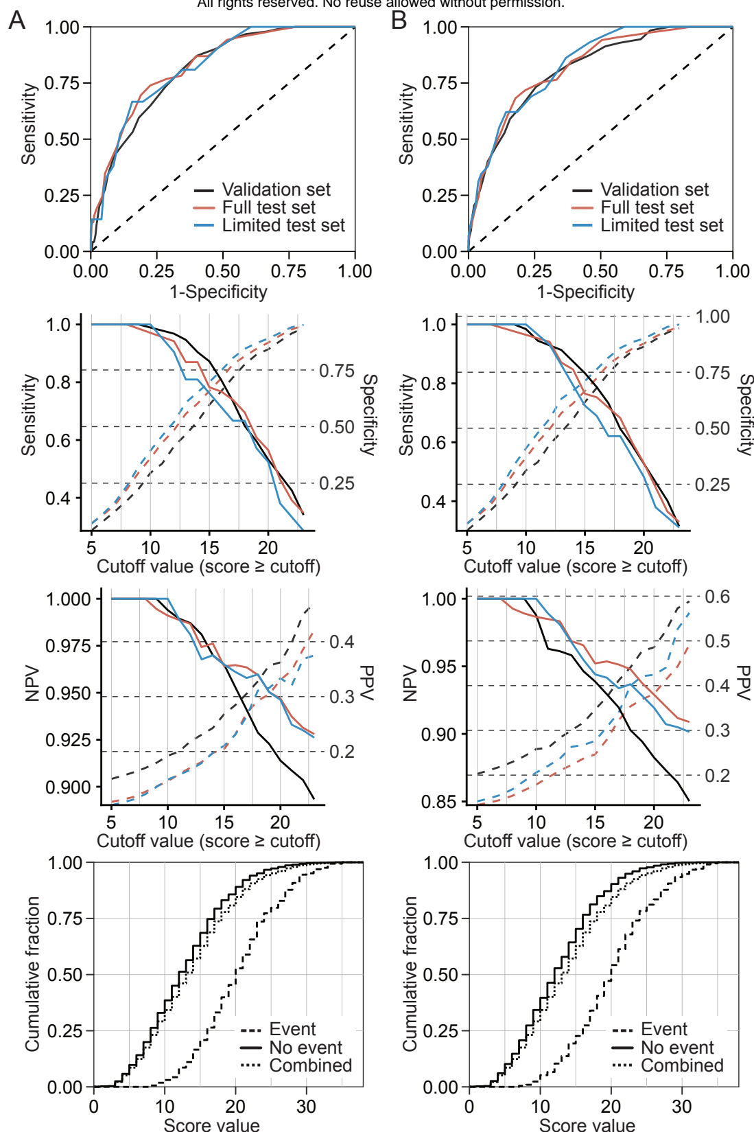
Figure 3. Summary of key characteristics of the score for predicting the combined endpoint of critical phase or COVID-19-related death (A) within 7 days of the diagnosis or (B) at any time point during follow up in the validation and test cohorts. Colour codes distinguish the different datasets as indicated. Sensitivity and NPV are indicated by continuous lines and the corresponding y-axis scaling on the left, while specificity and PPV are indicated by dashed lines and y-axis scaling on the right side of the respective panels. Bottom panels show cumulative fractions of patients meeting respective score cutoffs for a combined validation and full test set (combined n=1331). For all panels the median score (rounded to the next whole integer) of the imputations was calculated for patients with missing values.
