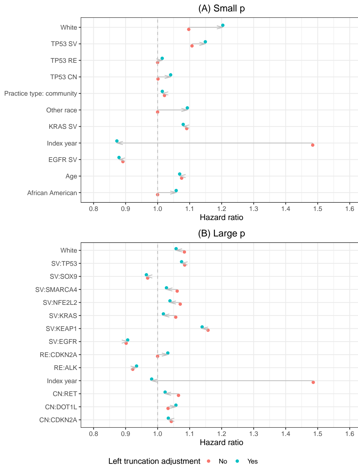
Figure 4: Hazard ratios from Cox lasso model
