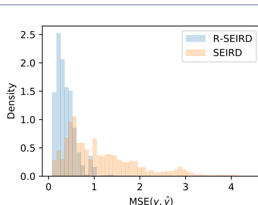
Figure 3: Comparison of prediction errors between R-SEIRD and SEIRD for the epidemic in the worst-hit county of each of the United States.
