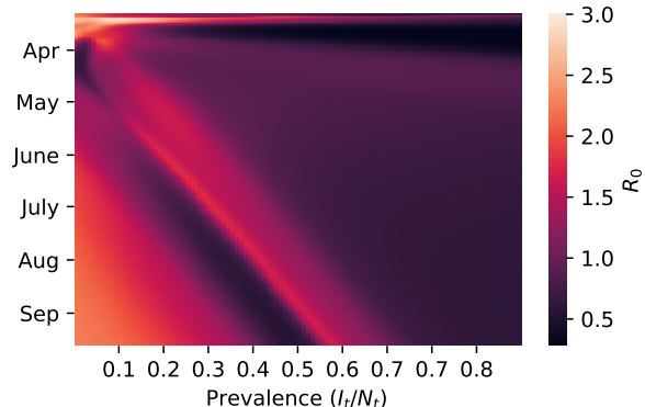
Figure 4: The learned mapping between time and prevalence to the infection rate.
