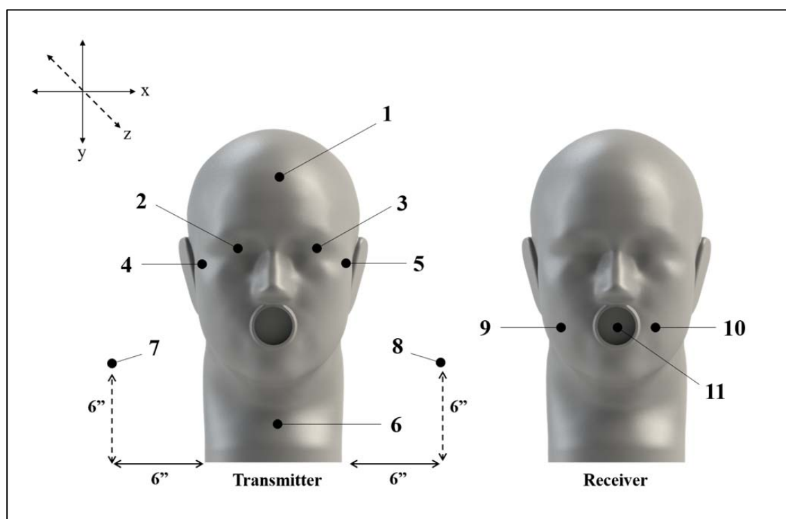
Figure 2. Headform Coupon Locations: 1) Forehead, 2) Left Eye, 3) Right Eye, 4) Left Cheek Bone, 5) Right Cheek Bone, 6) Neck, 7) Behind Left Shoulder, 8) Behind Right Shoulder, 9) Left Cheek, 10) Right Cheek, 11) Mouth.
