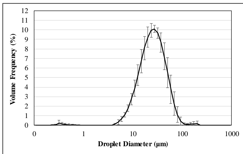
178 179 Figure 3. Mean Droplet Distribution for Triplicate Control Runs
