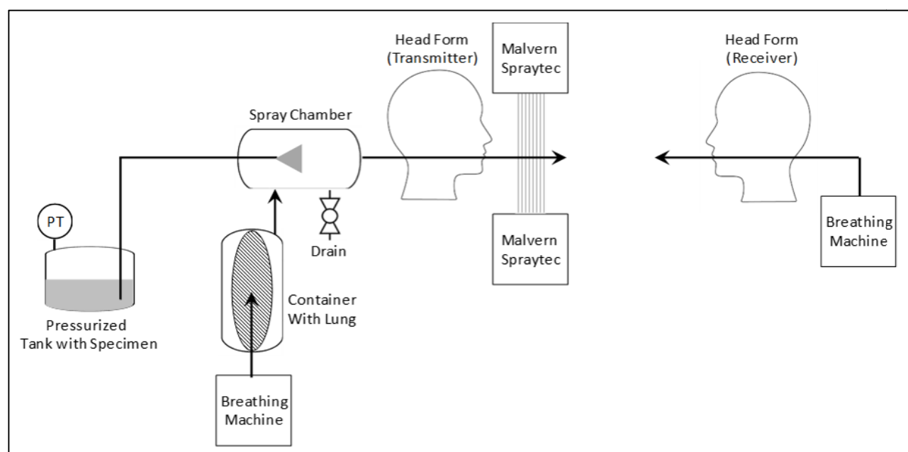
Figure 1. Droplet Transmission Test System Overview
