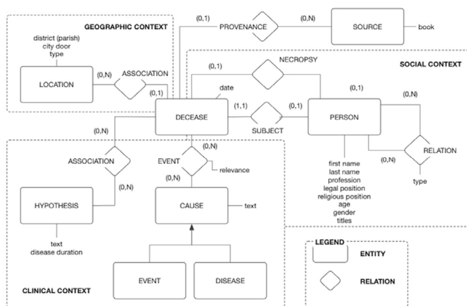
Fig. 3. Database structure.
