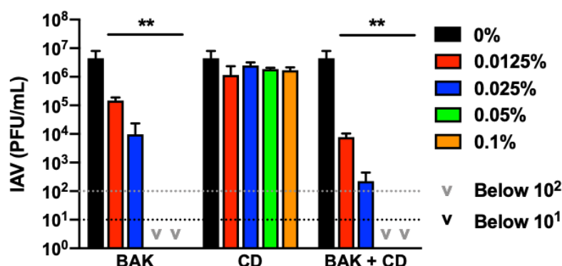
Figure 4. Viral inactivation by BAK and CD at concentrations less than 0.1%.
