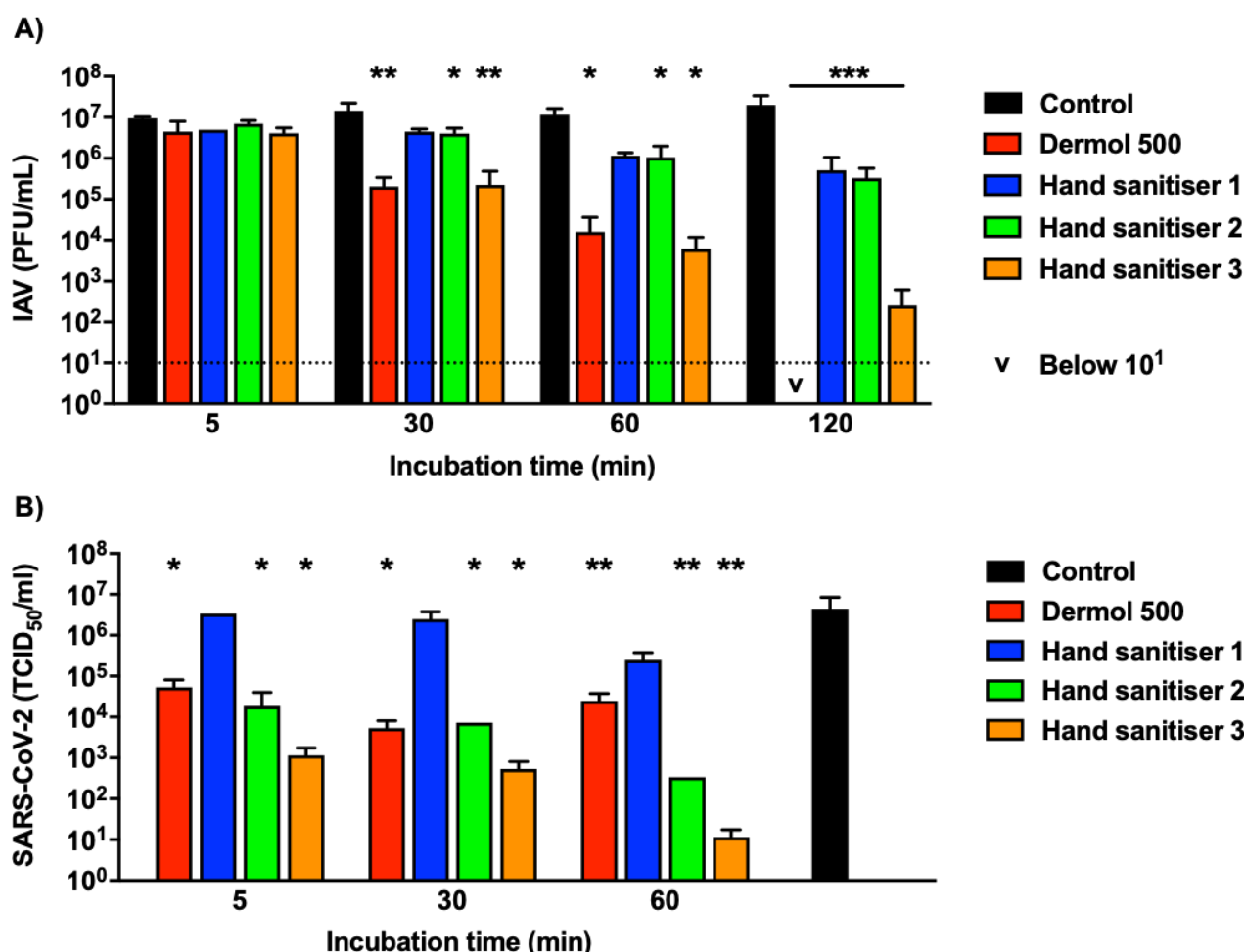
Figure 2. Dermol 500 lotion exhibits virucidal activity against IAV and SARS-CoV-2.
