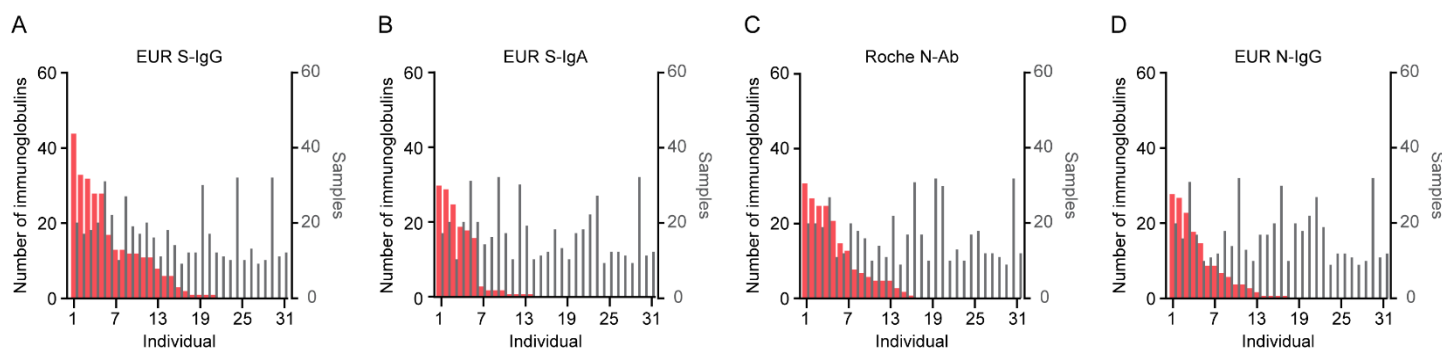
Fig EV7 - Proteins correlating to different SARS-CoV-2 antibody assays
