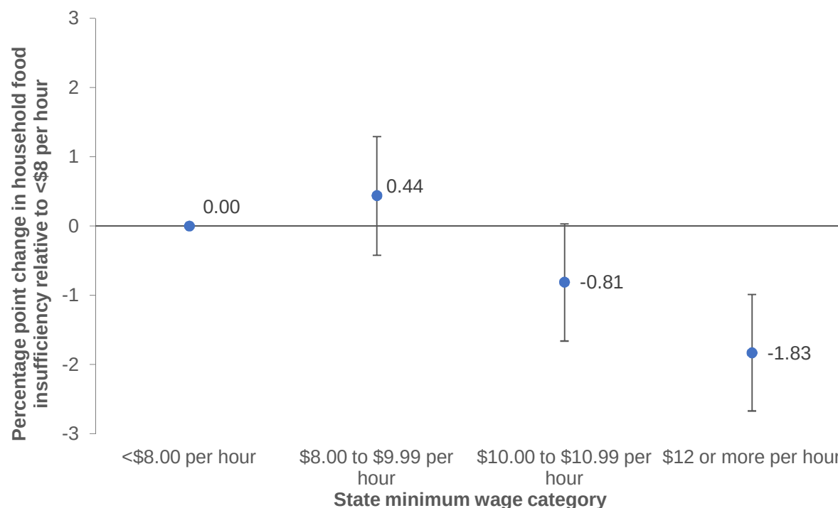
Figure 2: Marginal effect estimates of the relationship between state minimum wage, paid leave, and household food insufficiency among people younger than 65 years
