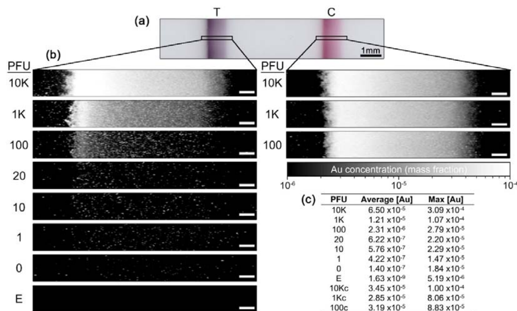
Figure 2. Mass fractions for viral dilution series (a) Digital microscopy image highlighting regions of interest within LFDs selected for subsequent synchrotron XRF measurements. (b) Au XRF images, expressed as mass fractions, on a common logarithmic scale are shown from the test and control strips from LFDs with descending PFU values. (c) a summary of quantitative values extracted from synchrotron XRF images, including average and maximum values within the image data.
