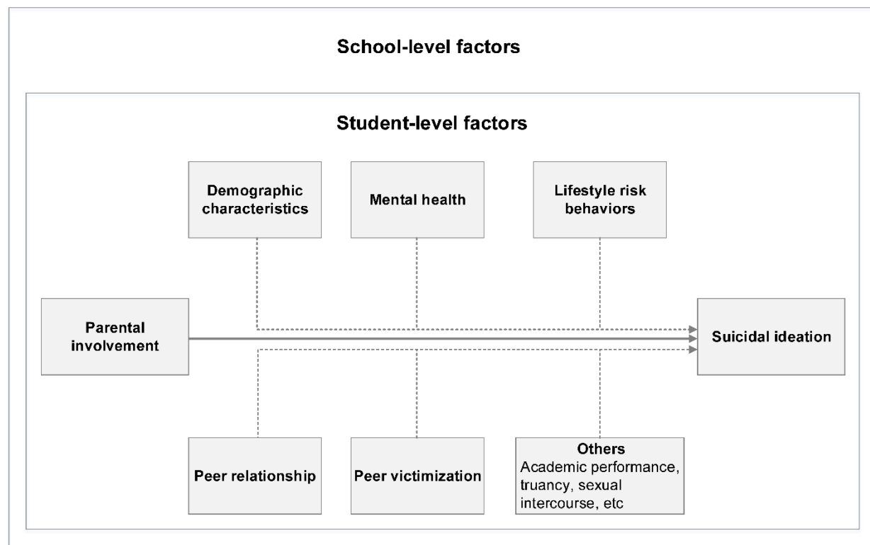
Fig. 1 Conceptual framework of the relationship between parental involvement and suicidal ideation among in-school adolescents in Vietnam
