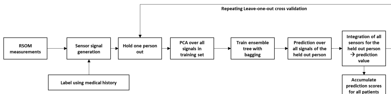
Figure 5. The machine learning pipeline consisting of an unsupervised component (PCA) and a supervised component (bagged ensemble trees). The dataset is obtained from the scan measurements and the labels are extracted from the medical history. The calculation of the PCA matrix as well as the training of the tree ensemble is performed on the training set only. Leave-one-out cross validation (LOOCV) is performed by repeating the training and evaluation process over all the patients and volunteers. For every person in the test set, the predictions are calculated for the trained tree ensemble on all the sensor signals. The average value of these predictions, called the predicted score, gives the final prediction value for the given person.
