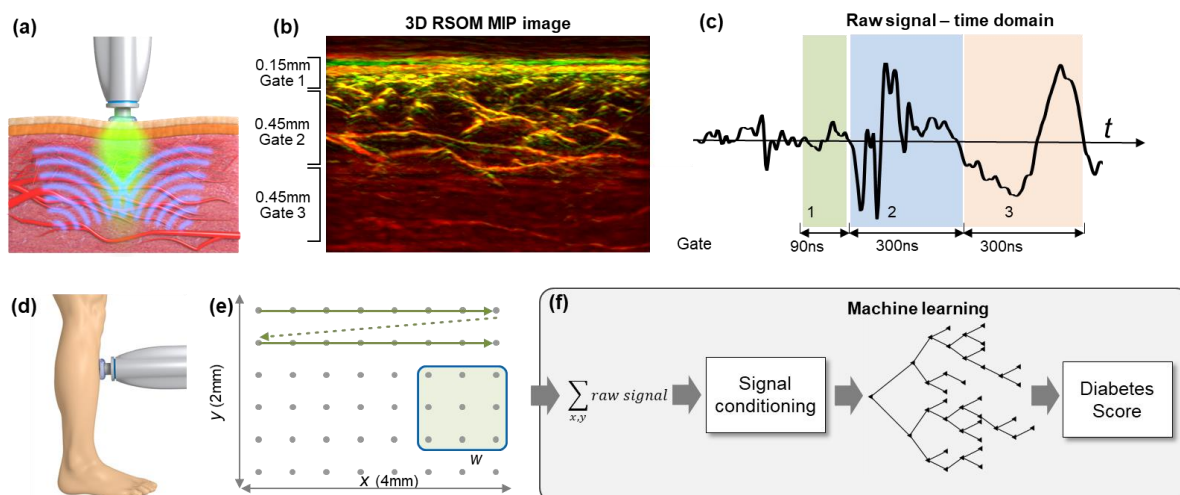
Figure 1. Machine-learning powered optoacoustic sensor. (a) The sensor is placed on the skin and simultaneously emits light into the tissue and collects generated acoustic signals emanating from different depths. (b) A 3D raster-scan optoacoustic mesoscopy (RSOM) reconstructed image, where the small veins dominate the epidermis region (corresponding to gate 1) and large veins are present in the dermis (gate 2 and 3). Gate 2 denotes the first part of the dermis and gate 3 corresponds to deeper regions. (c) A raw signal obtained using the optoacoustic sensor vs. time, where the 3 gates are shown with different colors. (d) A schematic depicting the location on the shin of patients where images are recorded by our in-house sensor system. The acquired time-series data is converted to sensor signals via integration in spatial windows of size w \times w , as depicted in (e). (f) Multiple sensor signals are generated for each patient. The sensor signals from all patients constitute the dataset. The dataset is annotated in terms of diabetes status using patients' medical history. Machine learning based on bagged ensemble trees is then performed in a supervised fashion to generate predictions about the diabetic status given the 1D optoacoustic sensor signal.
