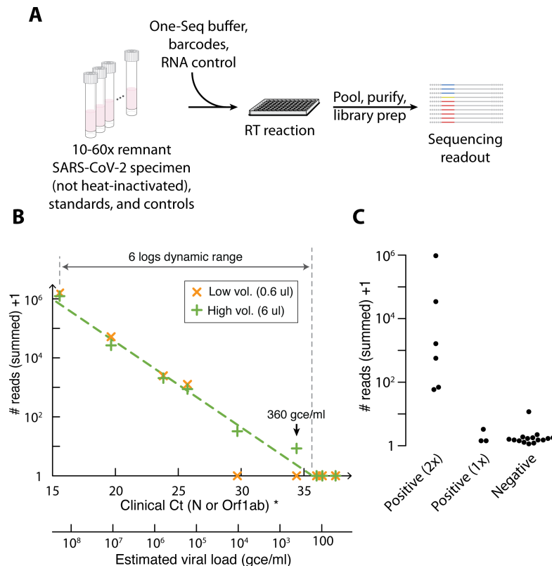
Figure 5 Validation of One-Seq on clinical SARS-CoV-2 specimens.
