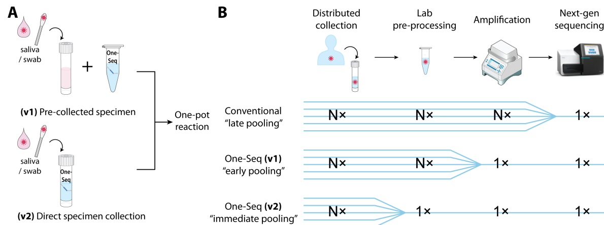
Figure 7 Potential clinical implementations for One-Seq. (A) Schematics for two clinical implementations: (v1) with pre-collected clinical specimen in viral transport medium, and (v2) with specimen collection directly into purpose-manufactured One-Seq collection tubes containing pre-assigned and uniquely identifiable sequence barcodes. (B) Compared with pre-collection (v1), direct collection (v2) completely avoids any liquid handling step and allows even higher scalability.
