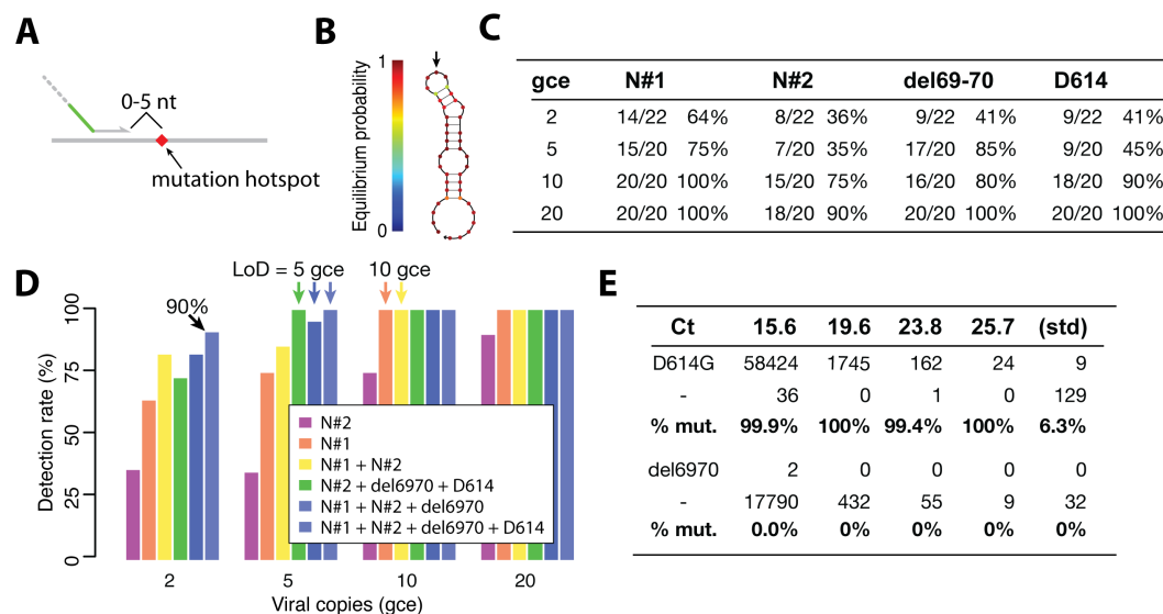
Figure 6 Multi-primer testing and variant sequencing. (A) Schematic for RT primer design targeting a viral mutation hotspot. (B) Example of strong local secondary structure in the viral genome that prevents efficient RT. Arrow indicates the mutated nucleotide. (C) Confirmatory sensitivity test results in contrived clinical samples for all four primer pairs (two in N gene and two in S gene for mutation sequencing) designed for One-Seq. (D) Comparison of detection sensitivity with different number and combination of primers. Combining more primers allows higher detection sensitivity, down to LoD = 2-5 gce with all four primers. (E) Viral sequencing showed all positive clinical samples we tested had D614G mutation, but none had the del6970 mutation, suggesting they were not related to the B.1.1.7 variant. Raw sequencing reads from four exemplary specimens as well as the virus standard sample (ATCC) were listed.
