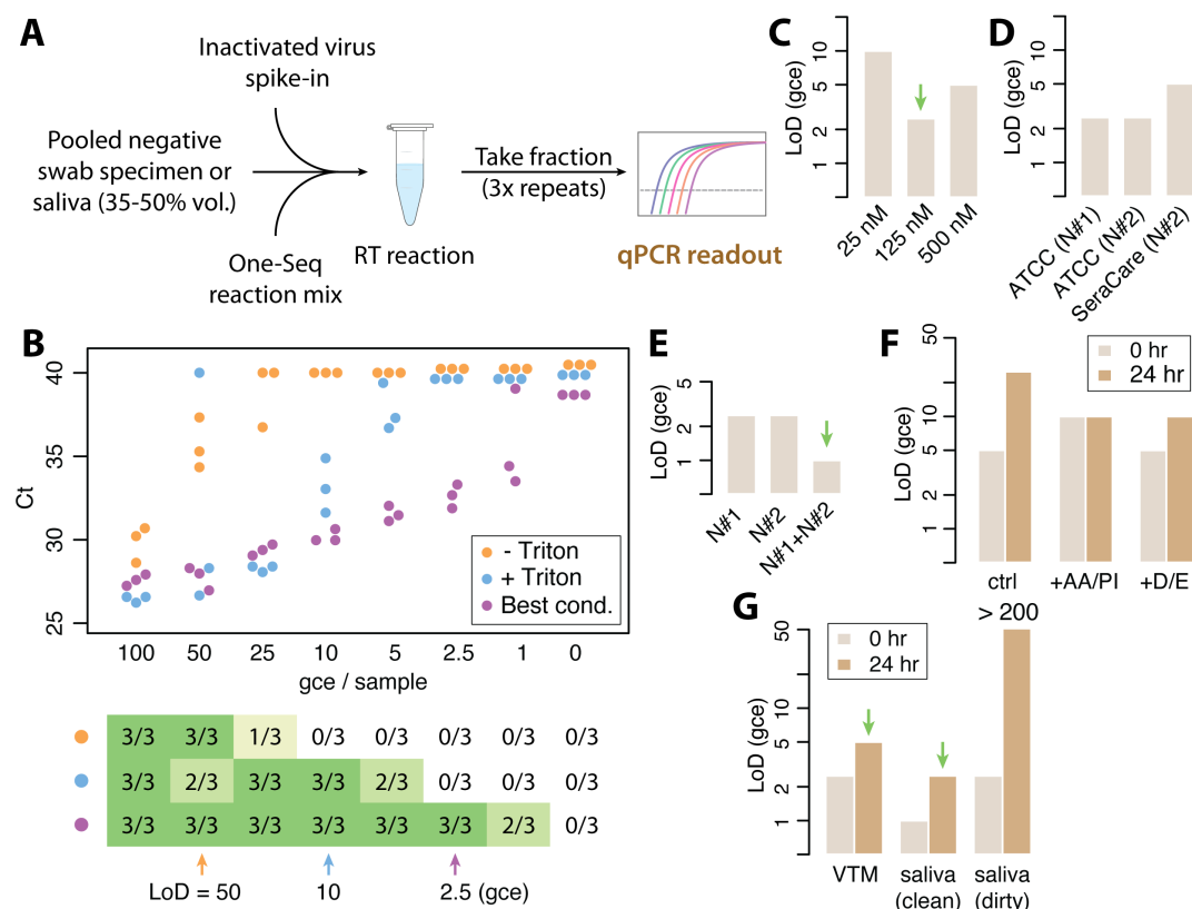
Figure 2 Development of an extraction-free, one-pot reaction for efficient viral reverse transcription and sample preservation. (A) Schematic of RT efficiency test in contrived clinical samples, using pooled negative specimen and inactivated virus spike-in. (B) Example of the RT sensitivity test, top, Ct values (3x repeats) plotted against different viral loads, in genome copy equivalent (gce), bottom, detection rate and limit of detection (LoD) determination. (C-E) RT sensitivity test under different conditions. (C) Comparison of different RT primer concentrations. (D) Comparison of different RT primers and validation with different virus reference standards. (E) comparison of single- vs dual-primer detection. (F-G) Effect of sample preservation buffer after incubation for 0 or 24 hr at room temperature in clean reaction buffer (F) or contrived patient samples (G). AA: antibiotic and antimycotic, PI: protease inhibitor, D: DTT, E: EDTA, VTM: viral transport medium.
