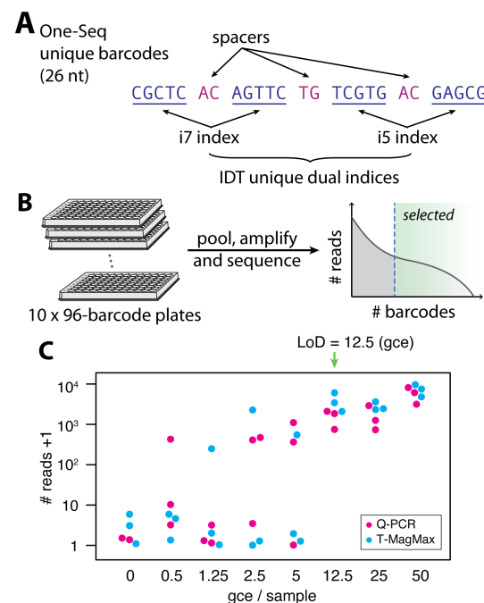
Figure 3 Barcode design and multiplexed sequencing sensitivity test. (A) Schematic of unique sample barcode construction. (B) Schematic for 960 sample pooling and barcode selection. (C) Example multiplexed sequencing sensitivity test and LoD determination, plotted as sequencing read count +1 against expected viral load. cDNA purification allows efficient library amplification after pooling.
