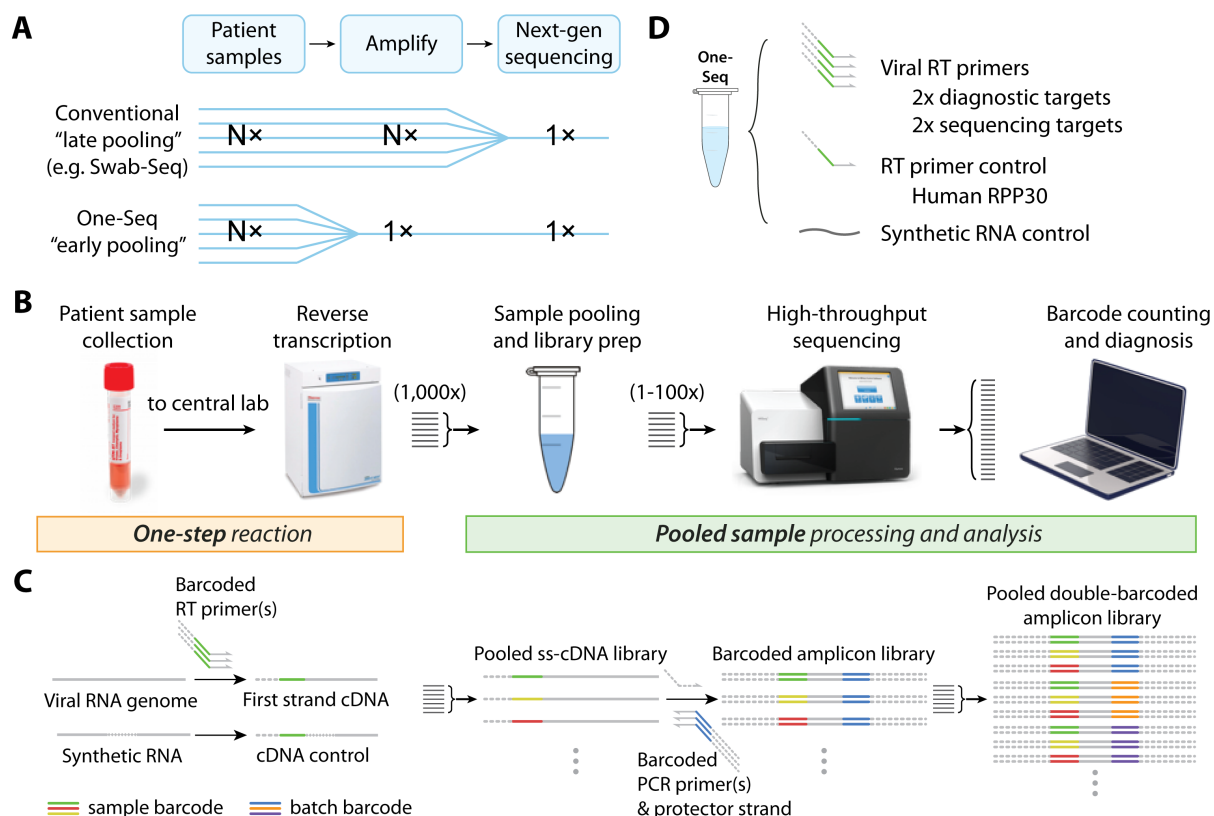
Figure 1 Principle and workflow of One-Seq for highly scalable viral detection and variant identification. (A) Illustration of One-Seq "early pooling" strategy in comparison with conventional "late pooling" methods. (B) Clinical workflow of One-Seq. Early pooling allows up to 100,000 patient samples to be pooled and analyzed together. (C) Molecular workflow of One-Seq. One-Seq uses upfront sample barcoding and a "protector" strategy to enable early sample pooling, and uses a two-stage pooling strategy to support highly scalable testing. (D) Illustration of One-Seq reaction components. One-Seq uses multiple RT primers for viral diagnostic and sequencing, one human gene RT primer and one synthetic RNA as positive controls.
