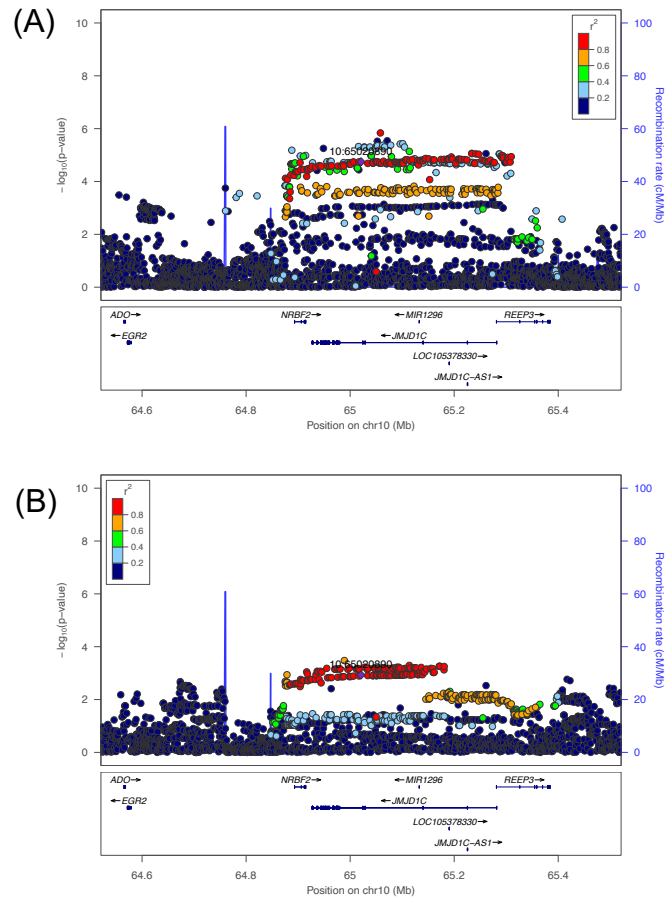
Figure S2. Association signal around NRB2/JMJD1C locus on chr10 in LAT and EAS cohorts.
