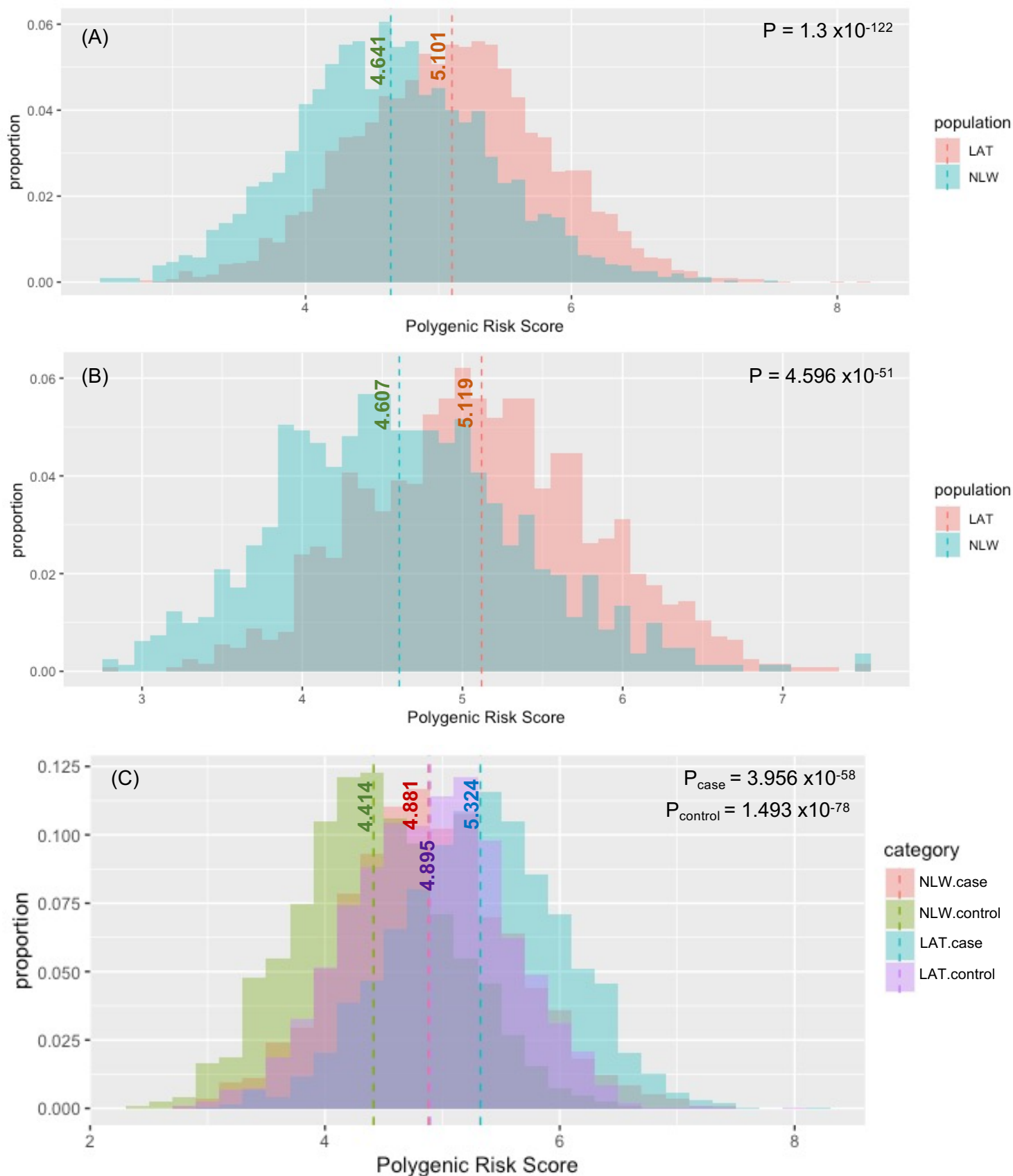
Figure 4. Polygenic Risk Score (PRS) distribution based on GWAS loci for ALL.
