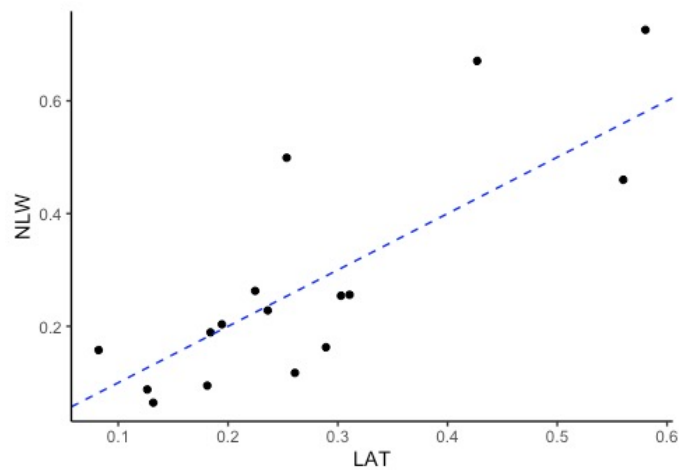
Figure S1. Effect sizes for lead SNPs in each of the 16 known loci. The effect size estimates (Beta) from GWAS in only the LAT or NLW subset from our discovery cohort are shown. The correlation coefficient ( r ) is 0.819. The dashed blue line is y=x .
