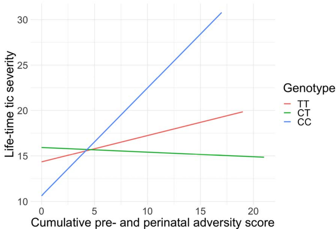
Figure 1: Interaction analyses of rs6539267 with a cumulative pre- and perinatal adversity score in relation to lifetime tic severity.
