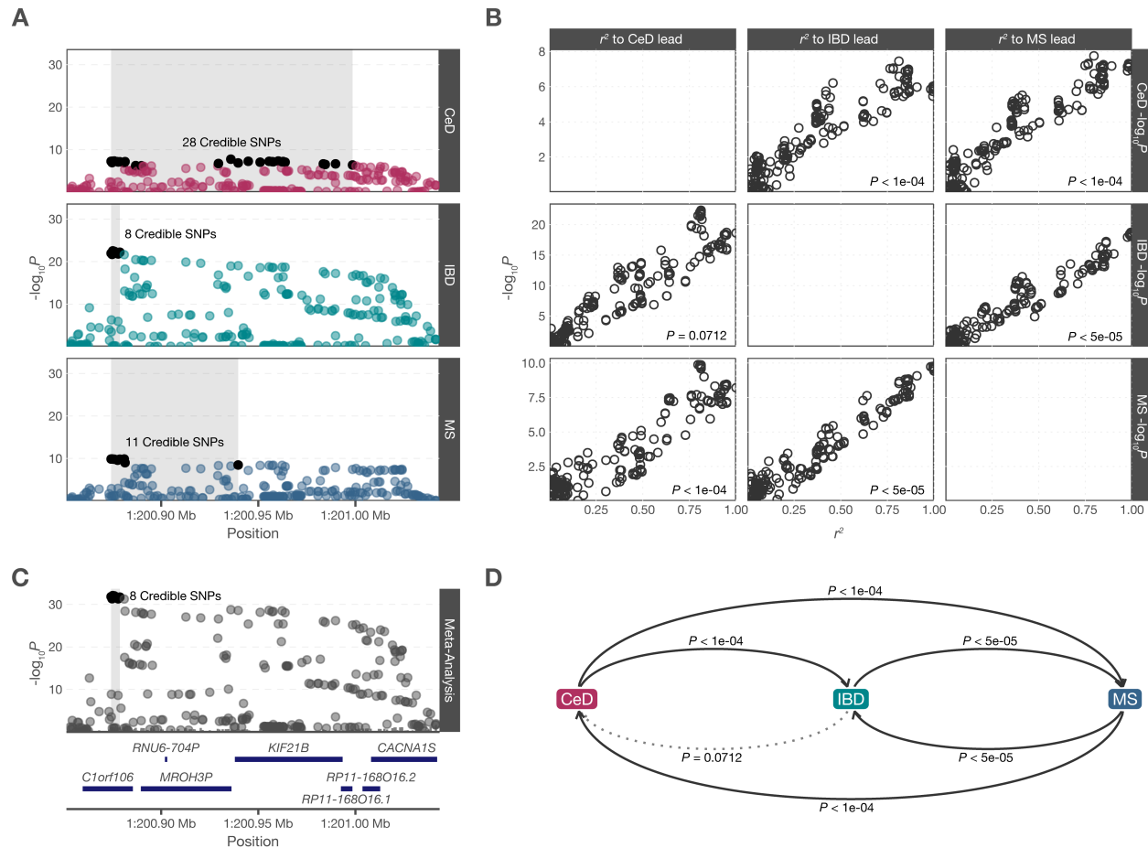
Fig. 2: A shared effect on chromosome 1 can be fine-mapped to eight variants across celiac disease, inflammatory bowel disease, and multiple sclerosis. (A) Overlapping associations in celiac disease, inflammatory bowel disease and multiple sclerosis on chromosome 1, with 95% credible intervals varying both in number of variants and physical span. (B) For each pair of diseases, the strength of association (vertical axis) for the first trait decays in a linear fashion as a function of r^2 to the lead SNP in the second trait, consistent with a shared causal variant. (C) Meta-analyzing across the three diseases gives in a stronger association signal, which can be fine-mapped to a narrow interval within C1orf106 . (D) We find strong pairwise evidence that the association is shared between all three diseases; JLIM is asymmetric, so we run comparisons in both directions.
