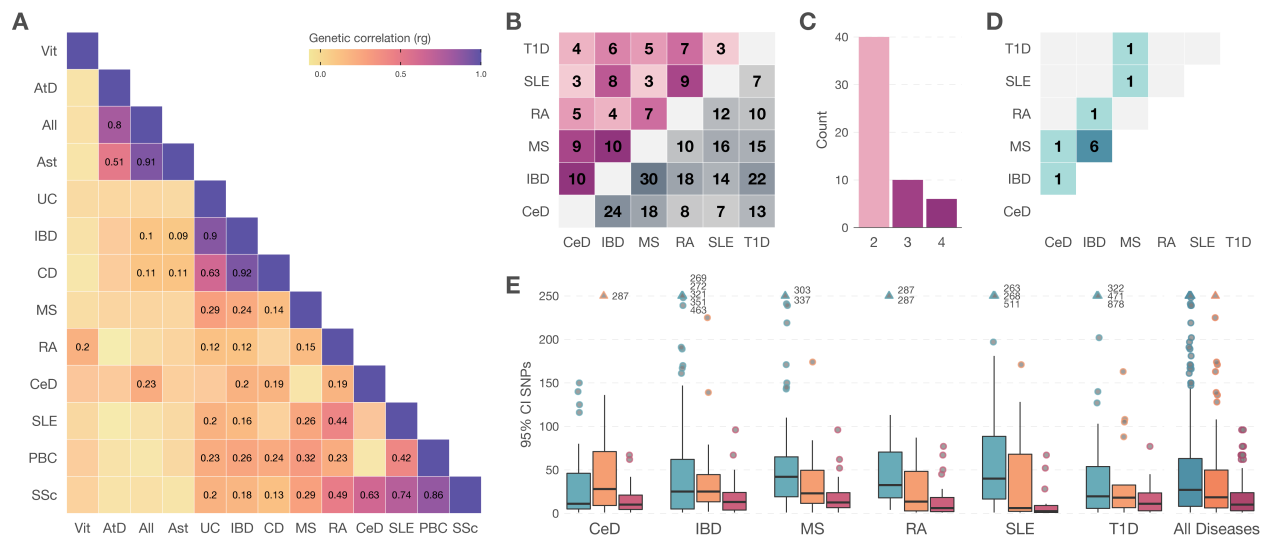
Fig. 1: Joint analysis of shared autoimmune disease risk alleles improves fine-mapping two-fold. (A) We find broad genome-wide correlation between association statistics for susceptibility to thirteen autoimmune and inflammatory diseases for which genome-wide association data were available (vitiligo, Vit; atopic dermatitis, AtD; allergy, All; asthma, Ast; ulcerative colitis, UC; inflammatory bowel disease, IBD; Crohn disease, CD; multiple sclerosis, MS; rheumatoid arthritis, RA; celiac disease, CeD; systemic lupus erythematosus, SLE; primary biliary cirrhosis, PBC; and systemic sclerosis, SSc). (B) This correlation is reflected in many loci harboring risk alleles to more than one of six diseases with available ImmunoChip data (lower triangle). Of these 236 pairs of associations, 99 are driven by the same underlying allele (upper triangle). (C) Risk alleles are mostly shared between two diseases (38 cases), with thirteen shared between three, and six between four diseases. (D) Twelve shared alleles have opposite effect directions, increasing risk of one disease and decreasing risk of another. This is most frequent between MS and IBD. (E) Combining cases and controls across diseases increases fine-mapping resolution for these shared associations. We assess resolution as the number of variants required to explain 95% of the posterior probability of association. This credible interval decreases by 58% when combining samples across diseases (red) compared to using only samples for one disease (orange). Associations that are not shared across diseases have similar credible interval distributions in individual diseases (blue).
