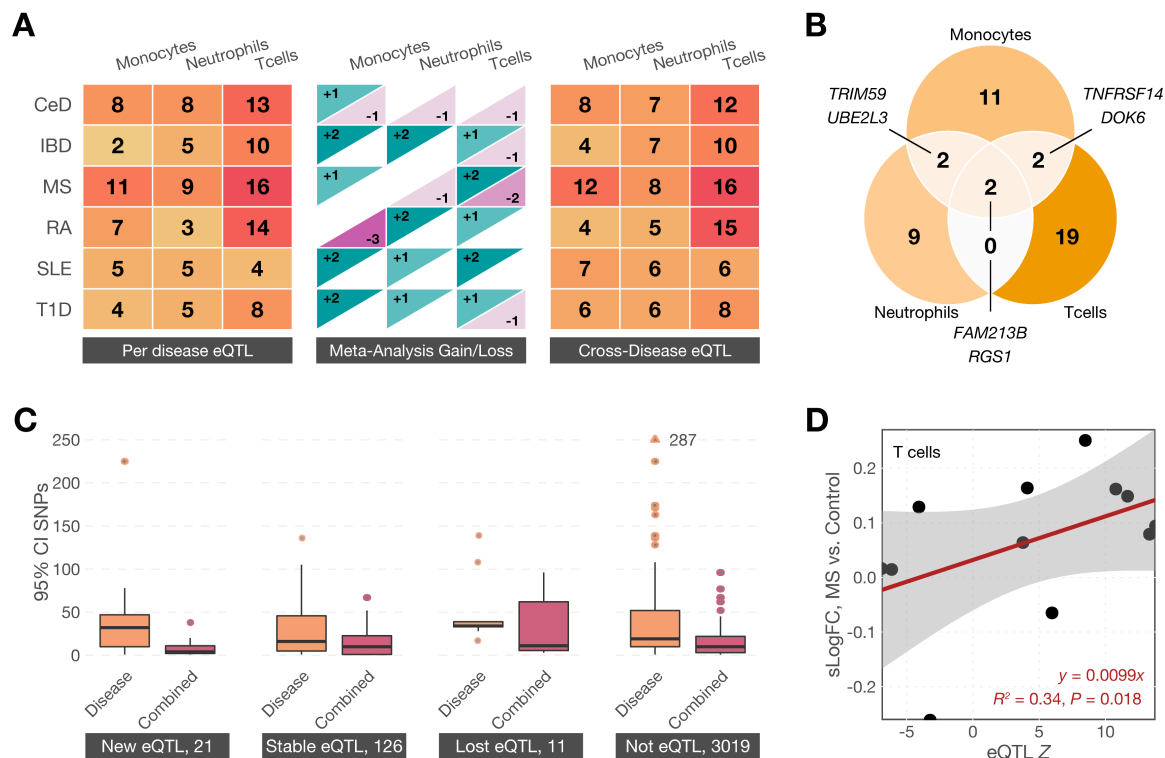
Fig. 3: The increased resolution of fine-mapping shared associations across diseases allows identification of more disease-eQTL overlaps. (A) We looked for shared effects between disease associations and expression QTLs in loci harboring shared disease effects. When considering each disease separately, we find 139 significant disease—eQTL overlaps across monocytes, neutrophils and T cells from the BLUEPRINT consortium (left panel). When comparing eQTLs to cross-disease meta-analyses, we find new overlaps (blue, middle panel) and no longer find evidence for some eQTLs (red, middle panel), for a grand total of 157 disease-eQTL overlaps (13% net discovery increase, right panel). (B) Some of the shared eQTL effects can be detected in multiple tissues, but most are restricted to a single cell type, indicating substantial effect specificity. (C) We find new eQTL shared effects in loci where the
