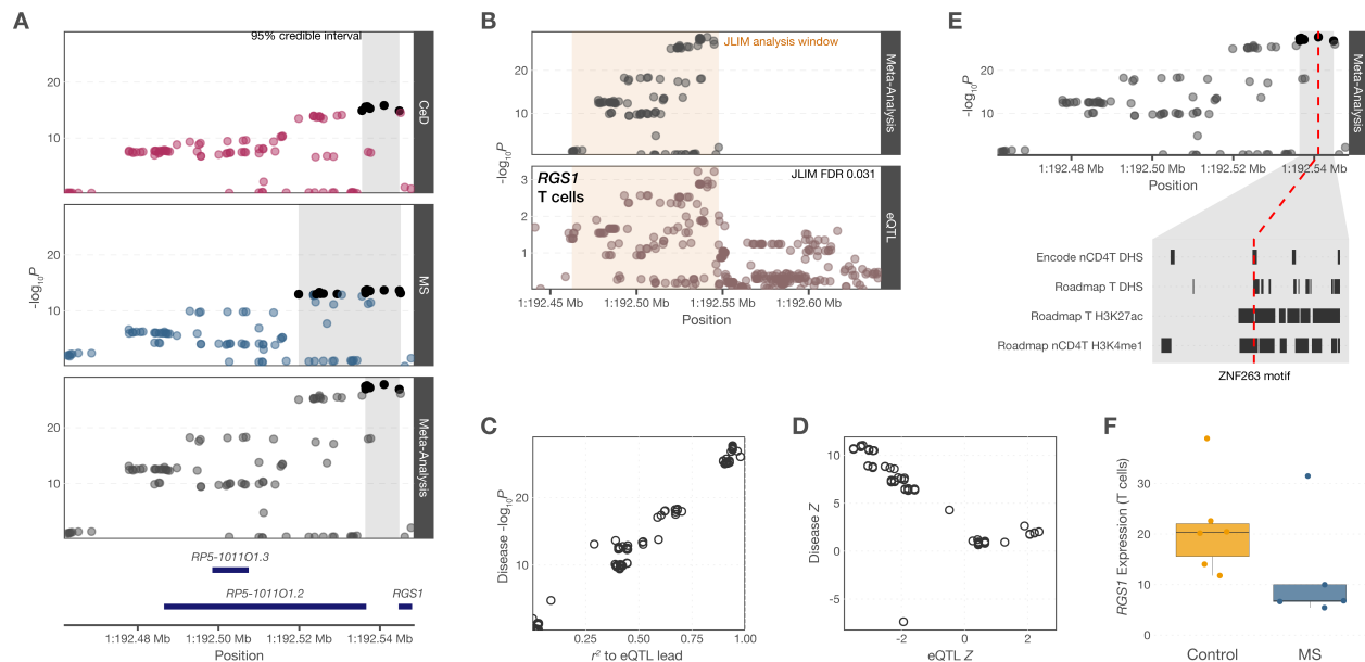
Fig. 4: Jointly analyzing an association shared between multiple sclerosis and celiac disease improves fine-mapping resolution and identifies a shared eQTL for RGS1 . (A) Overlapping associations for the two diseases are due to a shared effect (JLIM P = 5 \times 10^{-5} for CeD as primary trait; P < 5 \times 10^{-5} for MS as primary trait). Meta-analyzing across the two diseases increases the overall significance and a narrower credible interval (credible interval variants for each panel are in dark grey; the physical span of the credible interval is shaded grey). The credible interval focuses on the intergenic region proximal to RGS1 . (B) This shared association is also shared with an eQTL for RGS1 in naive CD4 T cells (JLIM P = 0.015 ). (C) The lead disease-associated variant lies in a region of accessible chromatin in naive CD4 T cells and total T cells. This is marked with H3K27ac in total T cells and with H3K4me1 in naive CD4 T cells, suggesting this is an active, primed enhancer element. (D) The RGS1 eQTL lead variant predicts the disease association P value, further indicating this is a shared effect. (E) Disease and eQTL association effects are negatively correlated, indicating that disease risk is associated with lower RGS1 expression.
