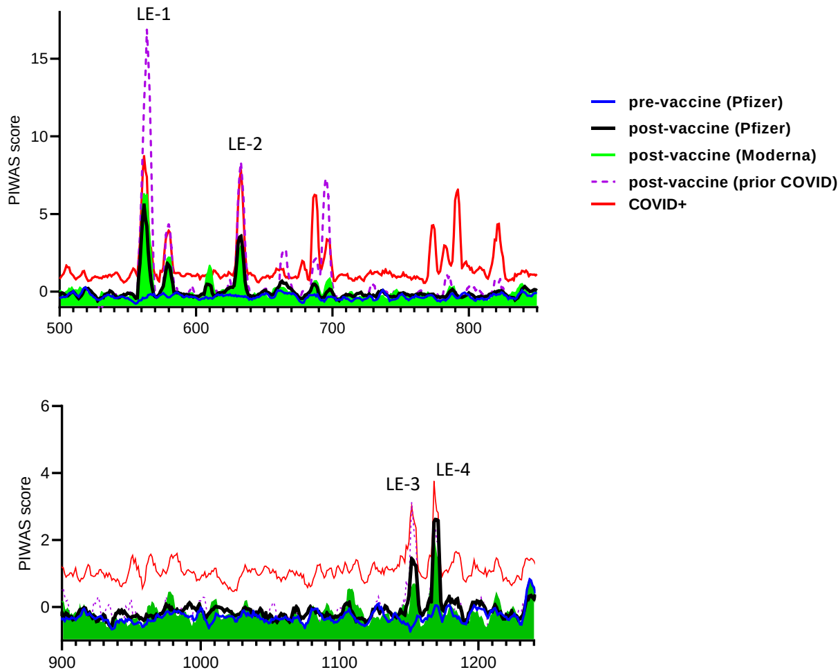
Figure 4. Dominant linear epitopes in COVID-19 mRNA vaccine recipients. The relative IgG binding (average PIWAS, Y-axes) to different linear epitopes (spike amino acid number, X-axis) is highlighted for the C-terminal domains of S1 (A) and S2 (B). Data are from N=20 Pfizer-BioNTech, N=8 Moderna vaccine recipients, and N=5 prior COVID-19 patients that received either Pfizer or Moderna vaccine as labeled in the key in upper right. The red line corresponds to the 95% quantile PIWAS score for a prior cohort of COVID+ subjects (12). Note the highest PIWAS scores for LE-1 and LE-2 as labeled and limited vaccine induced IgG towards fusion peptide region, aa 788-806 (40).
