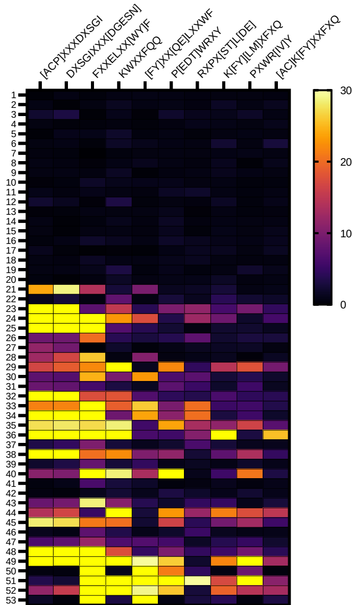
Figure 1. Heat map identifying amino acid motifs preferentially recognized by IgG from vaccinated subjects. Amino acid motifs were identified among the peptides immunoprecipitated by IgG from vaccine recipients using IMUNE algorithm and the level of enrichment (fold increase) in serum of individual subjects relative to pre-pandemic control subjects is depicted in the heat map. Samples 1-20 are pre-vaccine and samples 21-40 are the same subjects after Pfizer-BioNTech COVID-19 mRNA vaccination. Subjects 41-48 are from subjects that received Moderna vaccine. Samples 49-53 are vaccinated subjects that previously had COVID-19.
