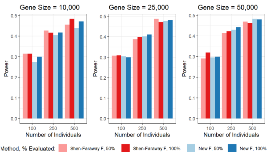
FIGURE A.1: A comparison of statistical power for the functional F-statistics when the genotype functions, G(t) , were evaluated at the locations of all of the included genomic variants versus half that number of equally spaced points.
