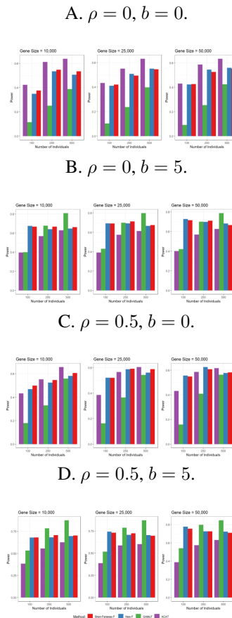
FIGURE 3: Statistical power for simulations assuming 5 continuous phenotypes, 5 causal variants, and causal effect sizes simulated from a normal distribution with \mu = 0 and \sigma_{\text{causal}} = 0.25 .
