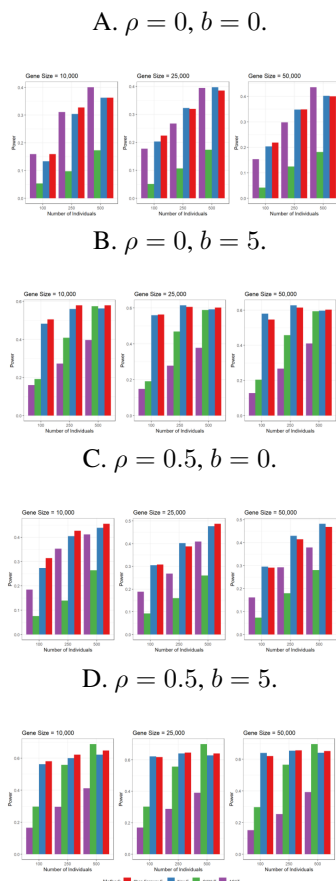
FIGURE 2: Statistical power for simulations assuming 5 continuous phenotypes, 5 causal variants, and causal effect sizes simulated from a normal distribution with \mu = 0 and \sigma_{\text{causal}} = 0.15 .
