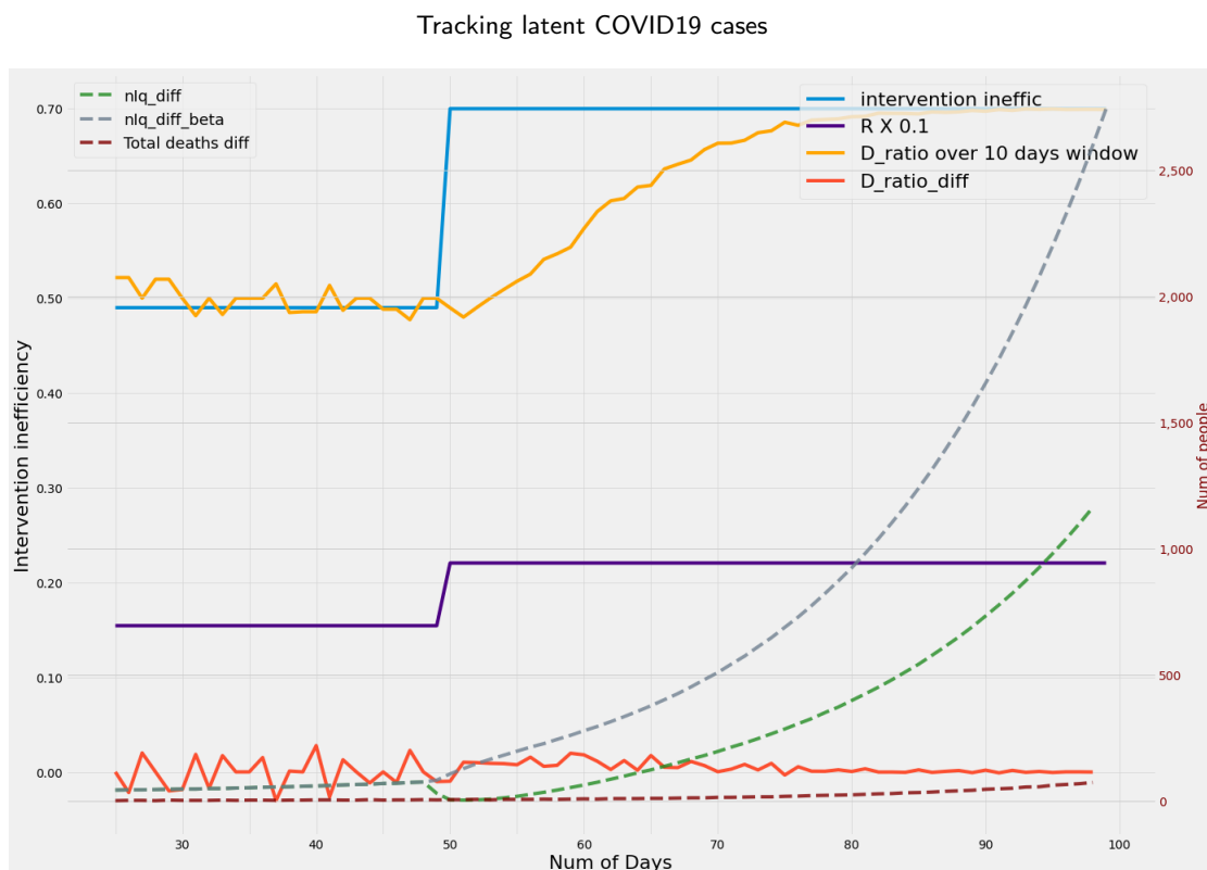
Figure 4: The graph considers the rise in active cases due to two scenarios, both of which result in identical changes in reproduction number R . When the rise in R is due to an increase in \beta , the active case increase yields a sharper curve giving a true indication of underlying cases. However, when the increase in R is due to increase in test-track-trace inefficiency, the rise in active cases are slower and in fact even decrease over the short term as the increasing cases are missed due to high inefficiency. A noticeable increase in active cases can only be seen past 30-40 days after the change. However, the increase in D_{ratio} is already evident in 10 days from the day inefficiency increases and stabilizes within a period of 20 days. Complete convergence as defined in Figure 4 comes around 35 days. It may thus be seen that the maximum convergence times of D_{ratio} metrics are comparable to the early rises in active case load based metrics. Thus windowed D_{ratio} based metrics are ideally suited as triggers for initiating mitigation.
