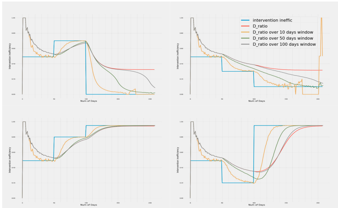
Figure 2: Variation of Intervention inefficiency and D_{smooth\ ratio} with time. The 4 plots show the trends in D_{ratio} over window periods of 10, 50 and 100 days when the inefficiencies are increased and decreased in different temporal orders. Metrics calculated with all window sizes show high day to day variation when the death numbers in either arm is very low. However, metrics with smaller window sizes are more prone to this daily variation. It is observed that D_{ratio} when smoothed over a small window of 10 days, converges faster but has a lot of variance due to daily fluctuations in numbers. Whereas D_{ratio} over a 100 days window length is smoother, but takes longer to make inferences due to slower convergence. Although sensitive to noise, 10 day window period gives the fastest convergence followed by 50 and 100 day periods.
