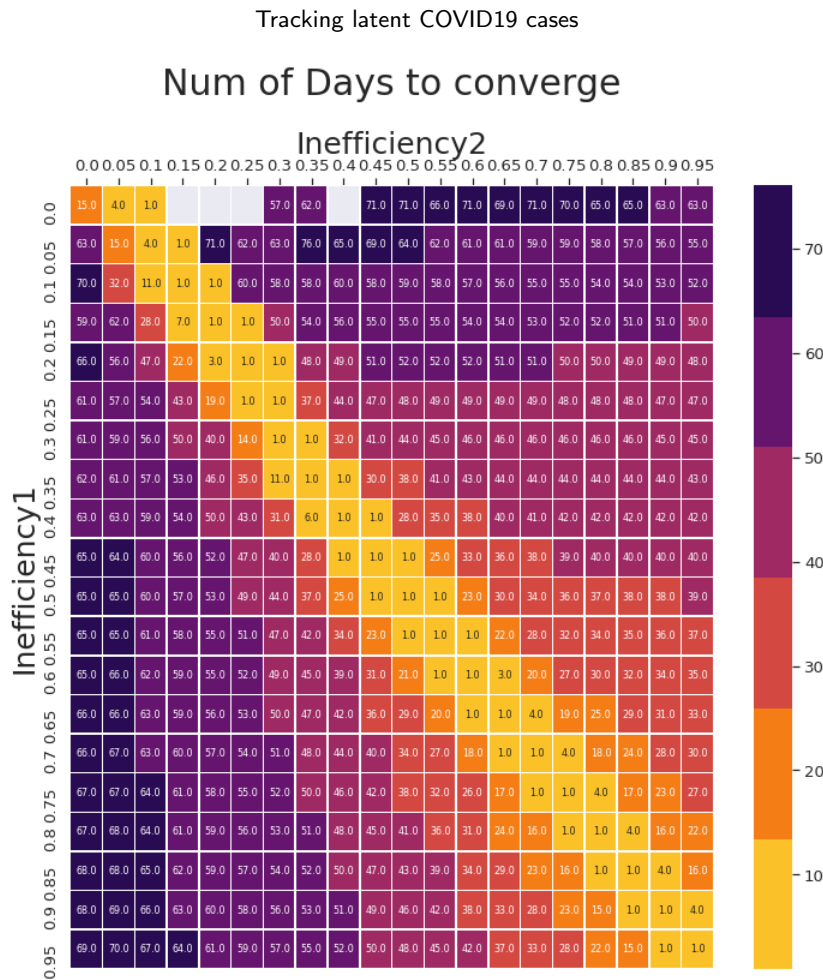
Figure 3: Correlation between Intervention Inefficiency_1, Inefficiency_2 when D_{smooth\ ratio} is calculated over a 50 day window and the number of days for D_{smooth\ ratio} to converge with Inefficiency_2 is plotted on a heatmap. The days to converge is the least on the diagonal and is largely symmetric. Transitions in the range of inefficiencies 0.2 through 1 converge within a period of 60 days and the range from 0.4 through 1 within 50 days. The empty (grey) cells indicate it takes more number of days to converge than the period of simulation or the cases are extremely low to show up in the D_{smooth\ ratio} . In general it may be seen that in the high inefficiency range where it is critical to react fast, the convergences are faster, thus emphasizing the utility of this metric.
