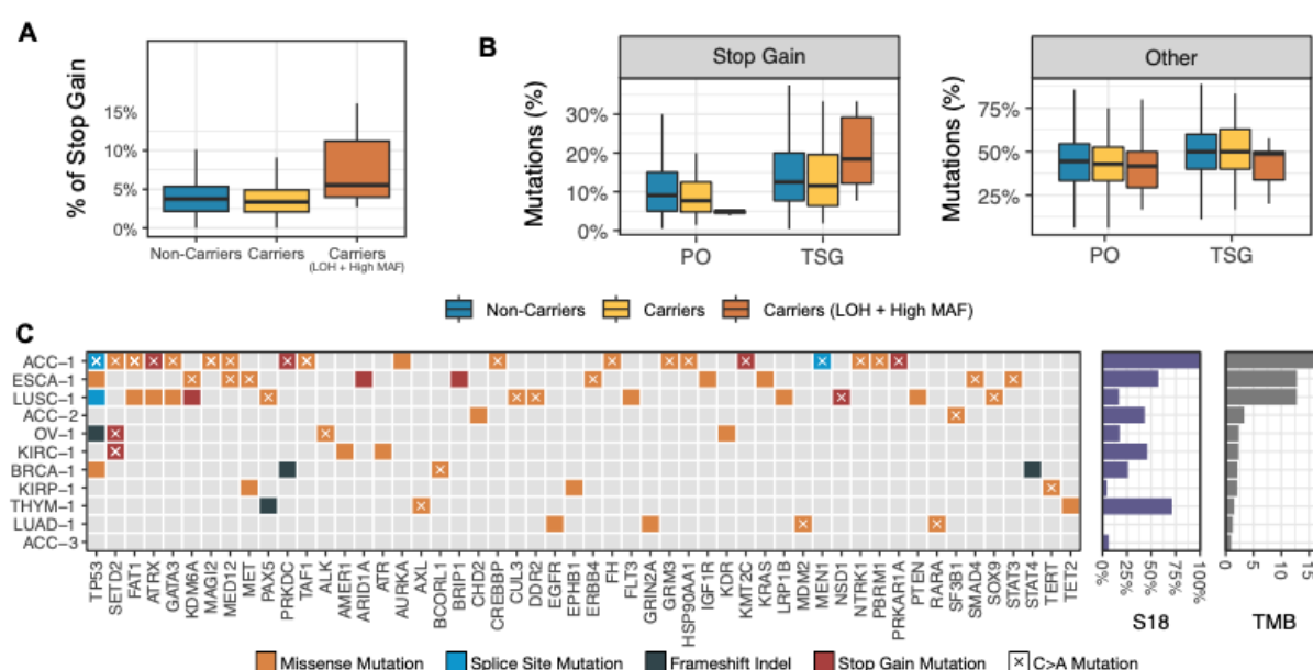
Figure 5. MUTYH potential stop-codon gain generation and frequent cancer gene mutations in the MUTYH variants carriers with LOH and High MAF. (A) Proportion of stop gain generating mutations in TCGA cohort. (B) Proportion of stop gain and other non synonymous mutations on cancer genes within TCGA's patients (PO: proto-oncogene, TSG: Tumor Suppressor Gene). (C) Co-mutation plot for the 10 damaging MUTYH variant carriers with LOH for the MUTYH region and with High MUTYH MAF in the tumor's RNA-seq quantification. Only displaying non-synonymous mutations in the cancer gene list evaluated by the FoundationONE panel. One sample (ACC-3) was removed because it lacked any cancer gene mutation. The right panel depicts COSMIC Mutational Signature 18 (S18) and Tumor Mutational Burden associated with each patient (Mutations/Mb).
