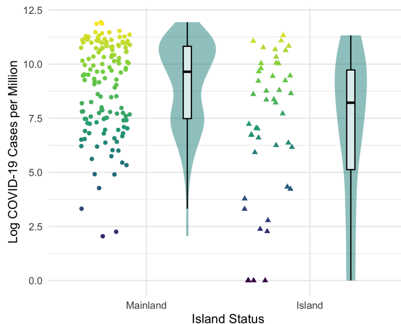
Figure 1. Log COVID-19 Cases per million of Mainland and Island Nations
