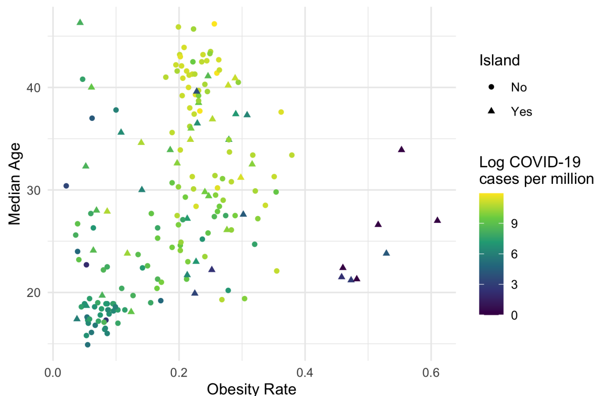
Figure 4. Association of Age and Obesity with Log COVID-19 Cases
