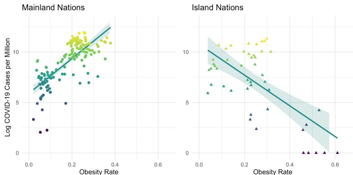
Figure 3. Interaction of Obesity Rate with Mainland and Island Nations
